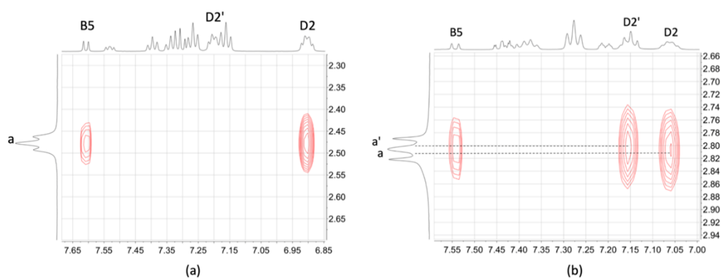
Figure 7. Part of the NOESY spectra (500 MHz, acetone- d 6 , 298 K) of (a) [Cu(xantphos)(1)][PF 6 ] showing NOESY crosspeaks between H a and H B5 , and H a and H D2 , and (b) [Cu(POP)(1)][PF 6 ] showing crosspeaks between the diastereotopic protons H a /H a' and H B5 , between H a and H D2 , and between H a' and H D2' .
