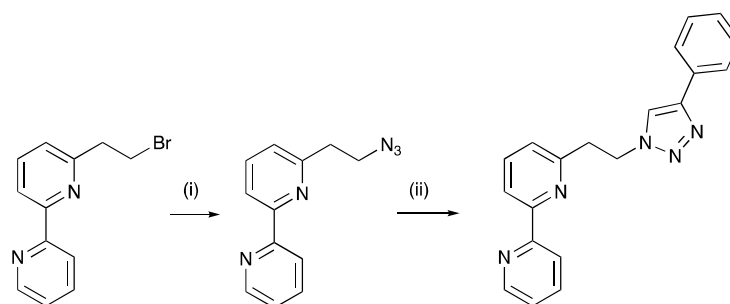
Scheme 3. Synthetic route to compound 3 . Reagents and Conditions: (i) \text{NaN}_3 , DMF, room temperature; (ii) phenylethyne, \text{CuSO}_4 \cdot 5\text{H}_2\text{O} , sodium ascorbate, t\text{-BuOH}/\text{H}_2\text{O} , 35\text{ }^{\circ}\text{C} . Yield = 54%.
