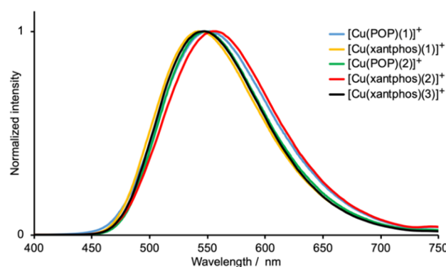
Figure 10. Normalized emission spectra of powdered samples of the heteroleptic copper(I) complexes ( \lambda_{exc} = 365 nm).
