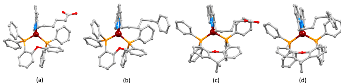
Figure 3. The energy minimized structures of the cations (a) [\text{Cu}(\text{POP})(1)]^+ , (b) [\text{Cu}(\text{POP})(2)]^+ , (c) [\text{Cu}(\text{xantphos})(1)]^+ and (d) [\text{Cu}(\text{xantphos})(2)]^+ .
