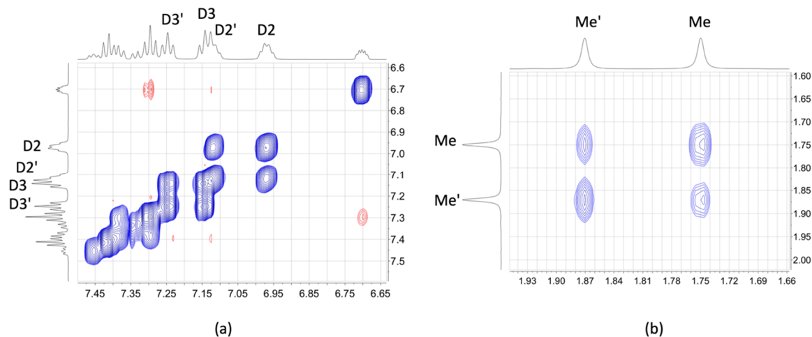
Figure 8. Part of the NOESY spectra (500 MHz, acetone- d_6 , 298 K) of [\text{Cu}(\text{xantphos})(3)][\text{PF}_6] . (a) The EXSY between \text{H}^{\text{D}2} and \text{H}^{\text{D}2'} , and between \text{H}^{\text{D}3} and \text{H}^{\text{D}3'} ; the EXSY peaks between \text{H}^{\text{D}4} and \text{H}^{\text{D}4'} are also visible close to the diagonal. (b) EXSY peaks between \text{H}^{\text{Me}} and \text{H}^{\text{Me}'} in the xanthene unit.
