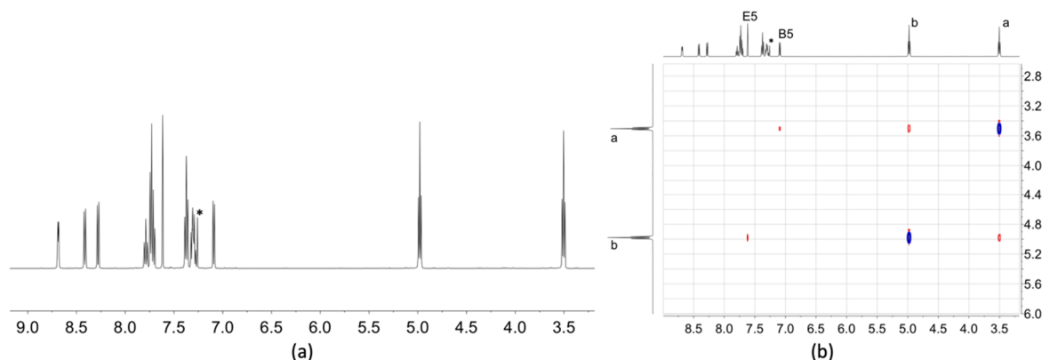
Figure 1. (a) The ^1\text{H} -NMR spectrum (500 MHz, \text{CDCl}_3 , 298 K) of compound 3 , and (b) part of the NOESY spectrum of 3 (500 MHz, \text{CDCl}_3 , 298 K). * = residual \text{CHCl}_3 .
