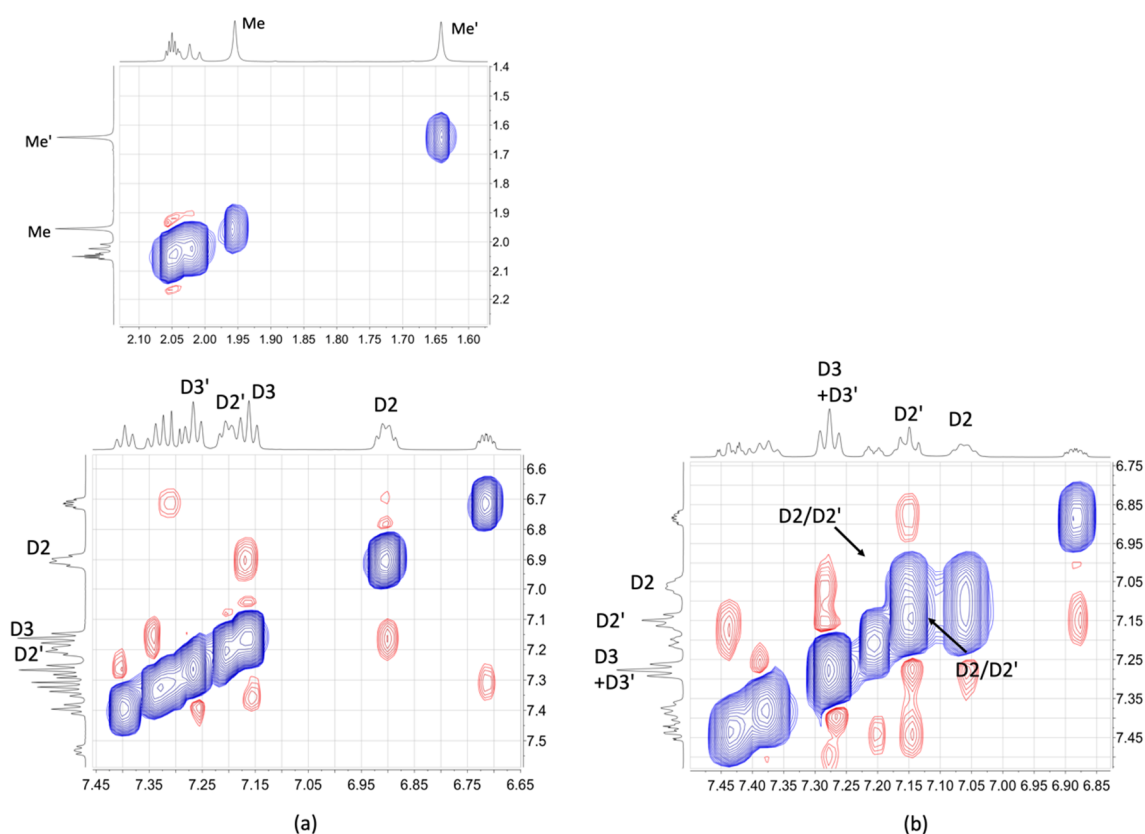
Figure 6. Part of the NOESY spectra (500 MHz, acetone- d 6 , 298 K) of (a) [Cu(xantphos)(1)][PF 6 ] with the methyl region shown at the top, and (b) [Cu(POP)(1)][PF 6 ]. EXSY peaks appear in the opposite phase (blue) to NOESY crosspeaks (red), and are observed between H D2 and H D2' in [Cu(POP)(1)][PF 6 ] but not in [Cu(xantphos)(1)][PF 6 ].
