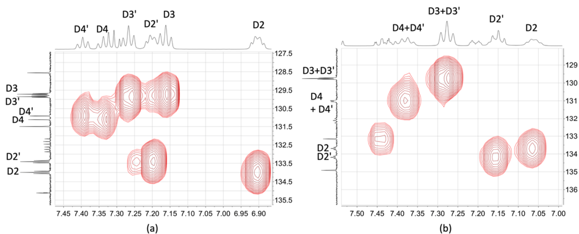
Figure 5. Part of the HMQC spectra ( ^1\text{H} 500 MHz, ^{13}\text{C} 126 MHz, acetone- d_6 , 298 K) of (a) [\text{Cu}(\text{xantphos})(\mathbf{1})][\text{PF}_6] and (b) [\text{Cu}(\text{POP})(\mathbf{1})][\text{PF}_6] .
