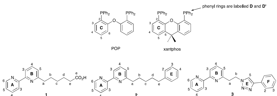
Scheme 1. Structures of the P ^ P and N ^ N ligands with labelling for the NMR assignments.
