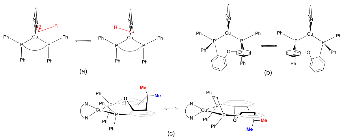
Scheme 4. Some of the possible dynamic processes in [\text{Cu}(\text{P}^{\wedge}\text{P})(\text{N}^{\wedge}\text{N})]^+ cations: (a) desymmetrization of the \text{P}^{\wedge}\text{P} ligand by conformational change of a 6-substituent when \text{N}^{\wedge}\text{N} = \text{bpy} , (b) conformational change of the POP backbone, and (c) inversion of the xanthene unit in xantphos which exchanges the positions of the methyl groups with respect to the O atom in the xanthene unit.
