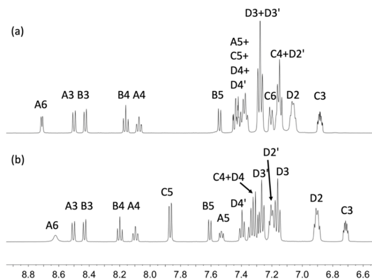
Figure 4. Aromatic regions of the ^1\text{H} -NMR spectra (500 MHz, acetone- d_6 , 298 K) of (a) [\text{Cu}(\text{POP})(\mathbf{1})][\text{PF}_6] and (b) [\text{Cu}(\text{xantphos})(\mathbf{1})][\text{PF}_6] .
