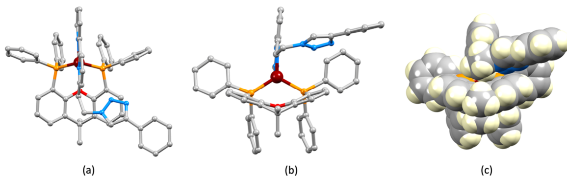
Figure 2. (a,b) Two views of the [\text{Cu}(\text{xantphos})(\mathbf{3})]^+ cation, and (c) a space-filling representation of diagram (b).
