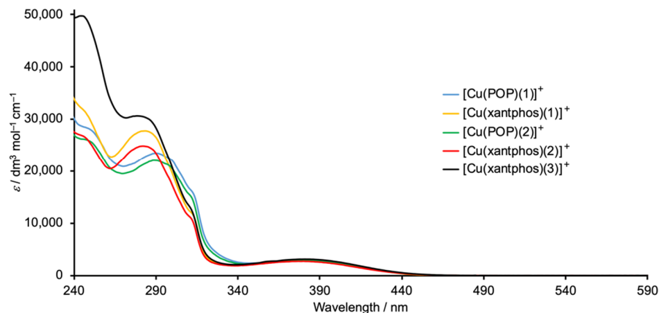
Figure 9. Solution absorption spectra ( \text{CH}_2\text{Cl}_2 , 2.5 \times 10^{-5} \text{ mol dm}^{-3} ) of the heteroleptic copper(I) complexes.
