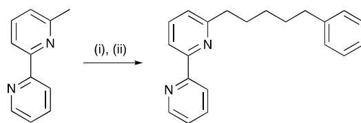
Scheme 2. Synthetic route to compound 2 . Reagents and Conditions: (i) Lithium diisopropylamide (LDA), THF, -78\text{ }^{\circ}\text{C} ; (ii) 1-bromo-4-phenylbutane, THF, room temperature. Yield = 30%.
