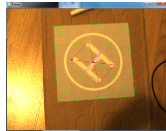
Fig. 17. Example of Output Image after the computer vision algorithm. In green, the heliport. In red, the H corners (maximum of signature). In purple, the minimum of the H signature
