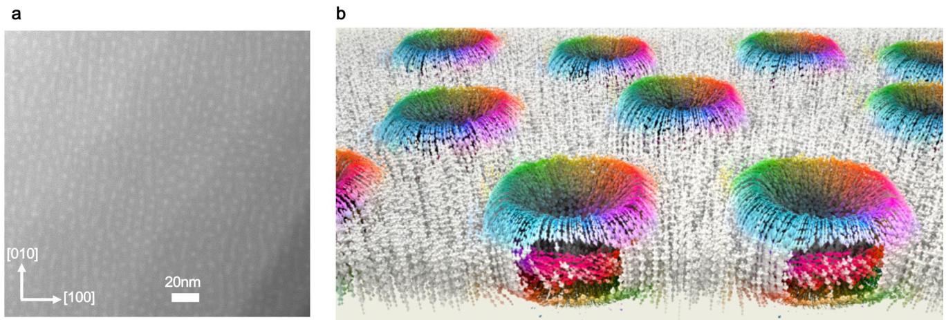
Extended Data Fig. 1 | Polar skyrmion structure in [(\text{SrTiO}_3)_{16}/(\text{PbTiO}_3)_{16}]_8 superlattice. a , Planar-view dark-field STEM imaging shows the widespread occurrence of nanometer-size ( \sim 8 nm) skyrmion formation along the [100] and [010] directions. b , Second-principles calculations of the skyrmion structure in the superlattice. The hedgehog-like skyrmion (Topological number +1) at the top and bottom interface between \text{SrTiO}_3 and \text{PbTiO}_3 , and the Bloch-like skyrmion (topological number +1) at the central plane in \text{PbTiO}_3 are clearly visible. The arrows represent the normalized electric dipole moments.
