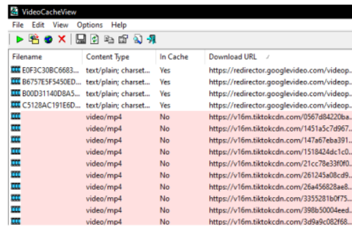
Figure 5. Video Cache View Acquisition
