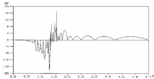
Fig.3. Errors of internal interpolation methods – example 2.
