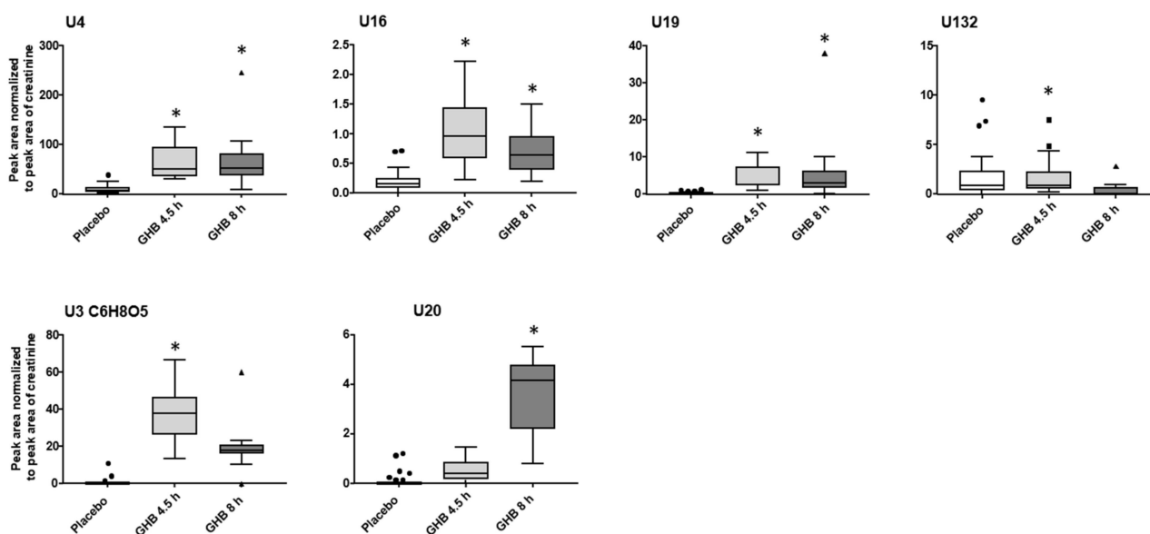
Figure 3. Box plots (outliers given as circles, squares or triangles for placebo, 4.5 h and 8 h post GHB intake, respectively) for selected promising, but still unidentified, compounds representing typically observed changes between placebo and two time-points after GHB intake. Depicted are analyte peak area to creatinine peak area ratios for placebo ( n = 34 ) and GHB groups after 4.5 h (Ut1, n = 19 ) and 8 h (Ut2, n = 15 ). Detection using univariate volcano plot analysis ( p < 0.05 and fc > 1.5 in at least 70% of the samples) is indicated by an asterisk.
