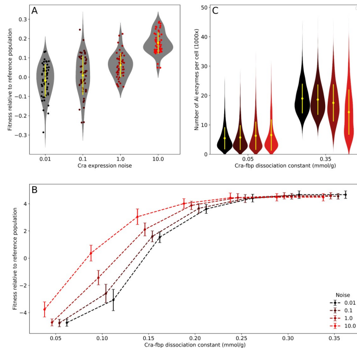
Fig 3. Cra expression noise increases fitness in a fluctuating environment when a population has low mean fitness. (A) Mean population fitness increases with Cra expression noise. We estimated fitness values by competing a population against a reference population with an intermediate level of Cra expression noise ( \eta^2 = 0.2 ) and the same Cra-fbp dissociation constant as the reference (0.1 mmol g -1 ), with 50 replicate simulations for each competition. In each replicate, both populations started with initially 1000 cells and grew together for four days in an environment with a constant flow of medium where the carbon source changed from glucose to acetate after two days. We estimated fitness from the change in the relative frequency of the non-reference population. Yellow diamonds and lines show the sample mean and one standard deviation. Circles represent the fitness values observed in each replicate, and grey violin plots are Gaussian kernel density estimates of the distribution of fitness values. (B) The fitness benefit derived from looser Cra-fbp binding is greater in populations with noisier Cra expression when the mean population fitness is low. We note that lower Cra-fbp dissociation constants correspond to greater binding strength. In this panel, fitness was determined through competition with a reference population that had both intermediate Cra expression noise ( \eta^2 = 0.2 ) and an intermediate Cra-fbp dissociation constant (0.125 mmol g -1 ), with 50 replicates for each competition. Circles denote mean fitness and are slightly offset on the horizontal axis for clarity. Error bars show one standard deviation. (C) Relaxing Cra-fbp binding increases the expression of the acetate incorporation enzyme Ai. We simulated cell growth on acetate in an environment with continuous medium through-flow for 21 days to equilibrate the population and then recorded the number of proteins per cell. Yellow diamonds and lines show the sample mean and one standard deviation. The violin plots are a Gaussian kernel density estimate of the distribution of proteins. The number of cells sampled for each combination of noise and Cra-fbp dissociation constant are 1637, 1619, 1835, 1719, 2005, 1991, 1981, and 2020.
