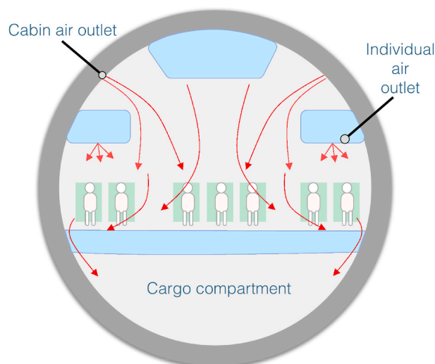
Fig. 1. Sample airflow, A320.
