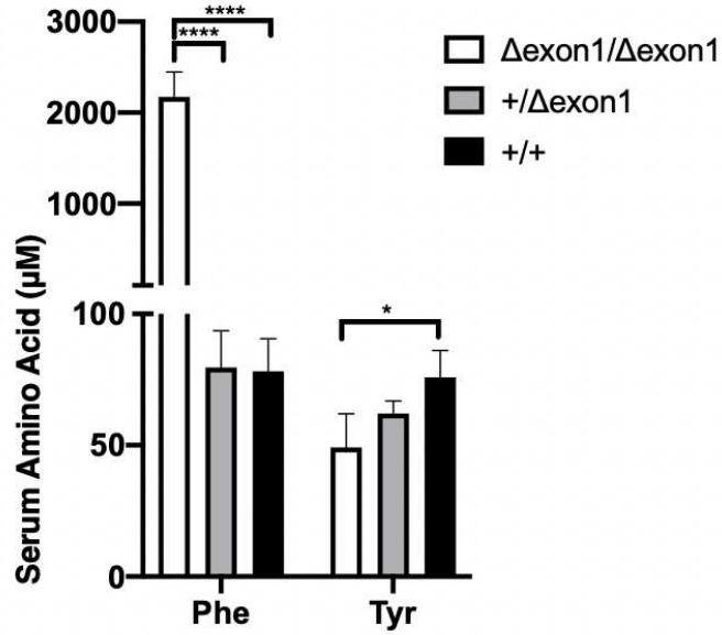
Pah \Delta exon1/ \Delta exon1 Pah +/ \Delta exon1
