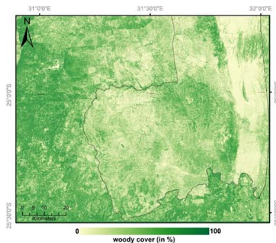
Figure 2. Sentinel-1 derived woody cover map of the southern part of the KNP with a spatial resolution of 10 m for the years 2016/17.
