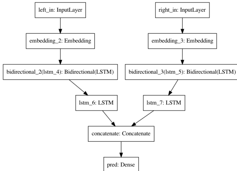
Figure 1: Dual-Input Encoder
