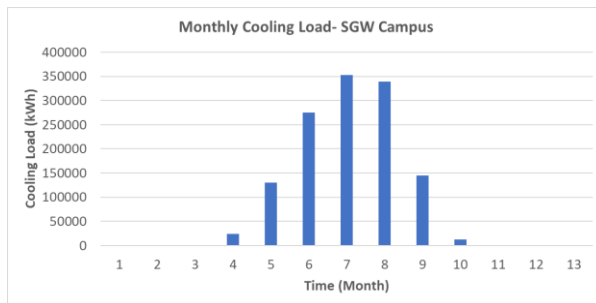
Figure 3. Simulation result of monthly Cooling demand of the buildings of SGW campus, Concordia University, Montreal.
