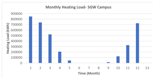
Figure 4. Simulation result of monthly heating demand of the buildings of SGW campus, Concordia University, Montreal.
