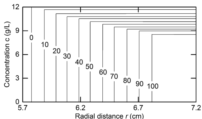
Fig. 1 Effect of radial dilution on the plateau concentration in simulated asymptotic (diffusion-free) sedimentation velocity distributions for a 12-g/L solution of equine \gamma -globulin ( s^0 = 7.38 \text{ S} , k = 0.00785 \text{ L/g} ) subjected to centrifugation at 60,000 rpm for the indicated times (min)
