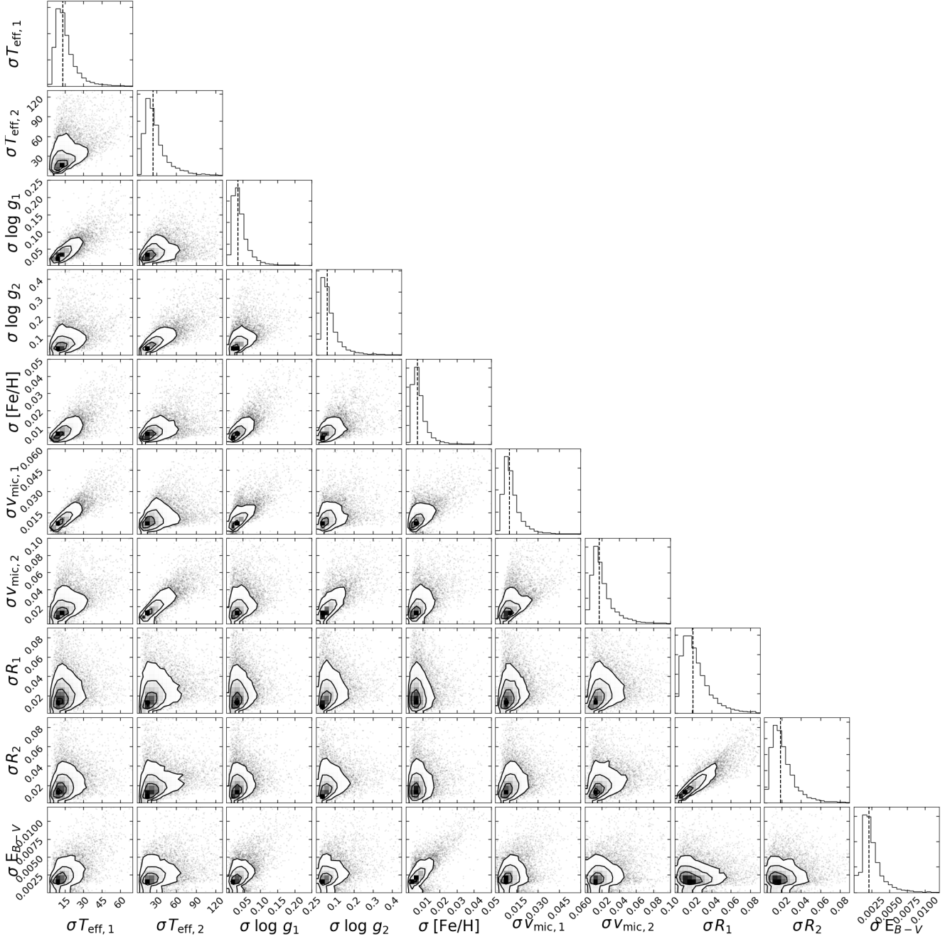
Fig. D.1. Ensemble of uncertainties of \theta parameters for the final sample of 12 760 analysed binary systems (see also Fig. 11). The uncertainty distributions are shown with diagonal panels, and the other panels indicate their correlations. The uncertainty units are those of the corresponding parameters (see Table 2). The tails of the distributions are truncated for clarity.
