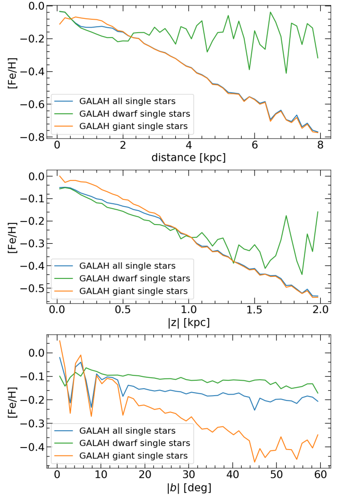
Fig. 19. Mean metallicity of GALAH DR2 single stars binned by distance ( top ), distance from the Galactic plane ( middle ), and absolute Galactic latitude ( bottom ). The GALAH DR2 single-star samples are those with \text{flag\_cannon} = 0 (Buder et al. 2018), and the dwarf-giant distinction following Zwitter et al. (2018). The sawtooth-shaped part of the lines indicates very few data points in the corresponding bins.
