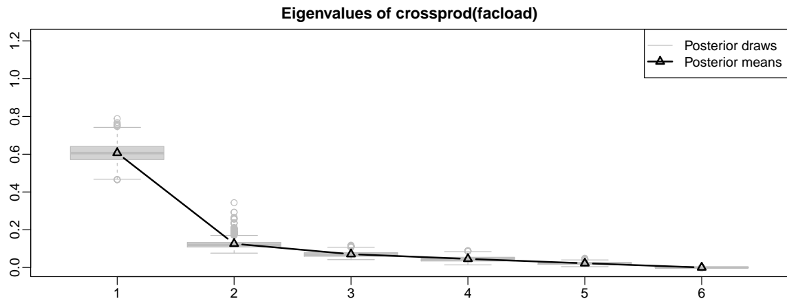
Figure 12: Eigenvalues of \Lambda^T \Lambda which can be used as a rough guide to selecting the number of factors.
