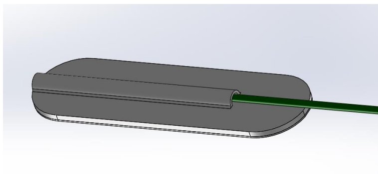
Figure 2.8: Paddle with added lumen to allow for stylet (green) to pass through
