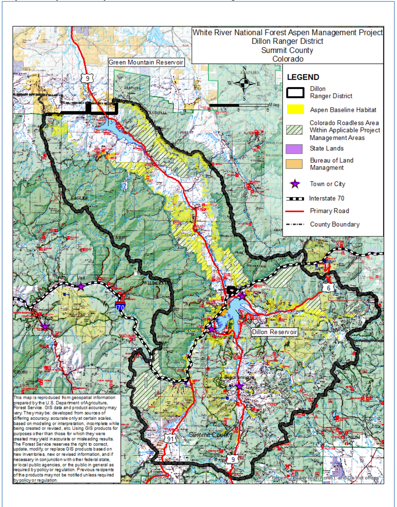
Map 9. This map shows the aspen baseline habitat, on the Dillon Ranger District, where activities could occur.
