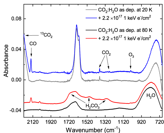
Fig. 5. MIR (2220–690 cm -1 ) FT-IR spectra of CO 2 :H 2 O (6:1) ice mixtures deposited at 20 and 80 K before (solid gray at 20 K and black lines at 80 K) and after (solid blue at 20 K and red lines at 80 K) 1 keV electron irradiation with a total fluence of 2.2 \times 10^{17} \text{ e}^- \text{ cm}^{-2} . The inset shows the difference spectra of the CO 2 :H 2 O (6:1) ice at 20 K after and before electron exposure.
