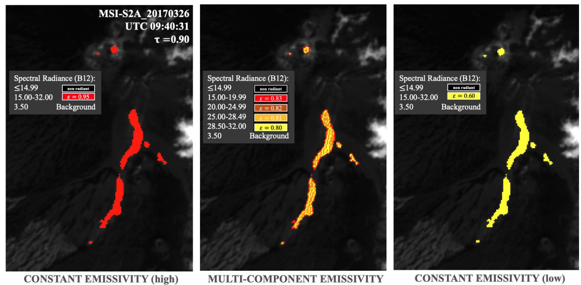
Figure 3.10 MSI scene (Sentinel 2A, Band 12) acquired on 26 March 2017, showing all radiant pixels, with recorded spectral radiance ( W \mu m^{-1} ), used for computation of total radiant heat flux at constant emissivity ( left ) 0.95 and ( right ) 0.60, as well as the ( centre ) multi-component emissivity approach (dynamic).
