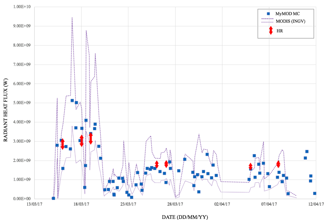
Figure 4.4 Comparison in computed radiant heat flux values from 15 March to 12 April 2017, derived from high-spatial resolution (HR OLI and Sentinel-2) and MODIS (MyMOD), using multi component approach, and MODIS (INGV), to derive min/max values, using constant emissivity (Wooster et al., 2003).
