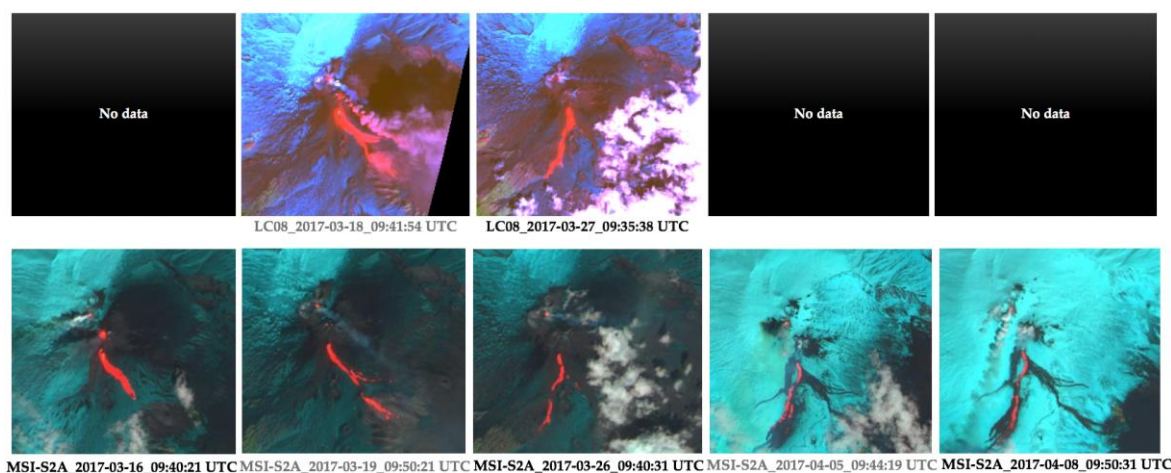
Figure 3.4 (top) Spaceborne scenes acquired by Landsat-8 (18/03/2017 and 27/03/2017) and (bottom) scenes acquired by MSI (16/03/2017, 19/03/2017, 26/03/2017, 05/04/2017 and 08/04/2017). Each panel displays an area of approximately 7 km 2 .
