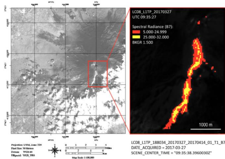
Figure 5. (a) Effusive activity recorded by Landsat 8 (Operational Land Imager (OLI)) on 18 March 2017 and; (b) 27 March 2017. Following the ‘two-component’ approach, cut outs in (a,b) contain ‘threshold’ values used in this study (Section 2.3.1), based on radiance values, where radiant pixels in red are used for computation of crust temperatures (i.e., emissivity 0.95) and radiant pixels in yellow, relating to the melt temperatures (i.e., emissivity 0.60). Background (BKGR) value (averaged radiance value of the pixels surrounding thermally anomalous pixels) was subtracted from radiance data (all thermally anomalous pixels), so that thermal component alone (excluding reflected radiances of daytime images in short-wave infrared (SWIR)) can be analysed.
