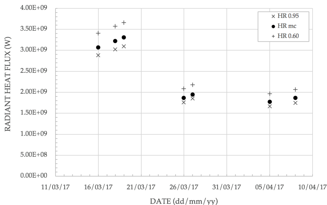
Figure 3.14 Radiant heat flux results (difference) using different emissivity values; (i) constant values (0.95 and 0.60), and (ii) multicomponent emissivity (HR mc). ‘HR’ signifies high-resolution data (combined OLI and Sentinel-2A spaceborne scenes).
