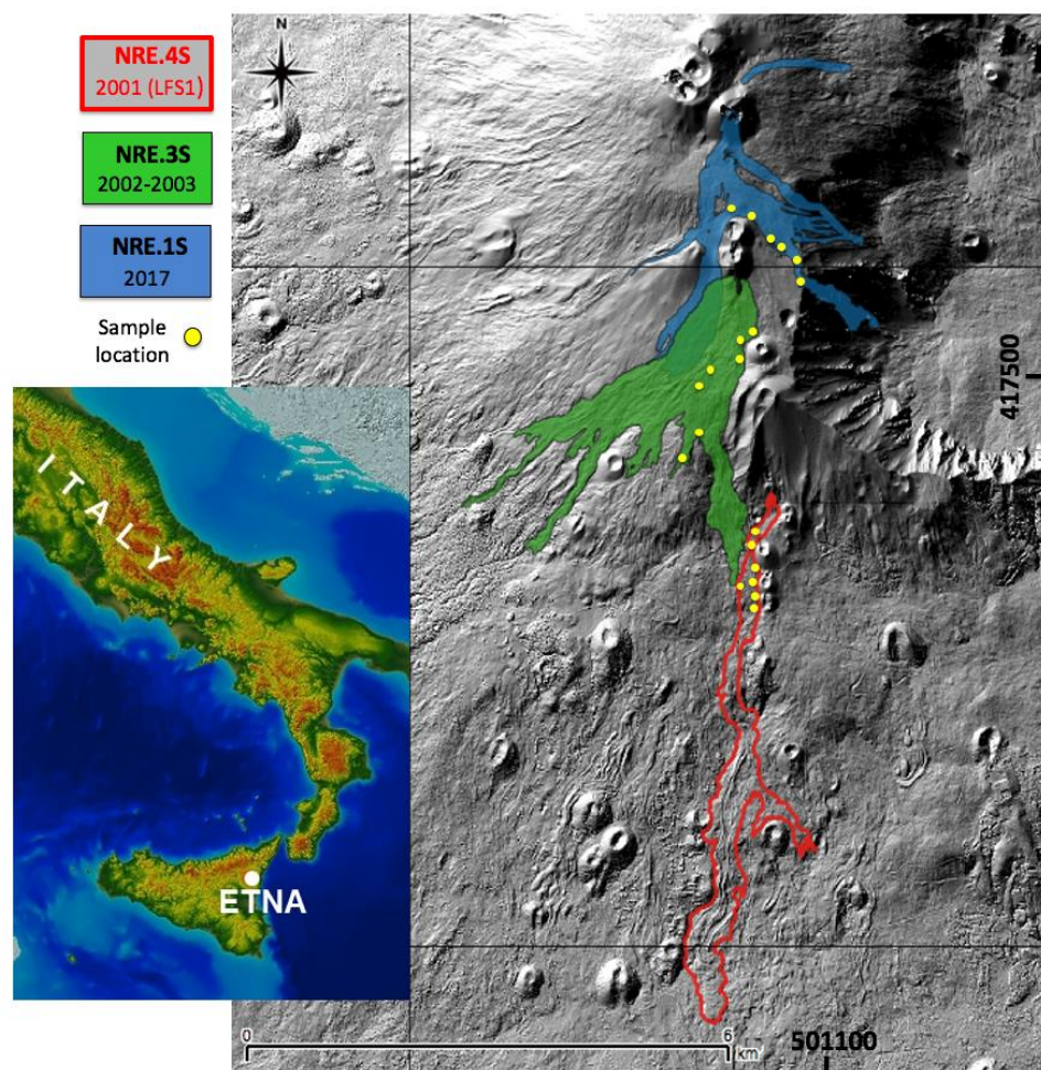
Figure 1.3 (main) The location and actual extent of the 2001 (red), 2002–2003 (green) and 2017 (blue) lava flows are shown on Mt Etna Digital Elevation Model (DEM); (inset) a geological map of Sicily, Italy (Tarquini et al., 2007) and the location of Mt Etna volcano. Approximate location of collected samples (NRE.1S, NRE.3S and NRE.4S) are indicated with filled yellow circles. Note that only LFS1 (Coltelli et al., 2007), individual lava flow (18 July–09 August 2001) was used for the 2001 eruption analysis.
