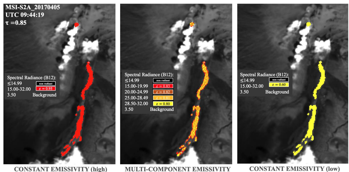
Figure 3.11 MSI scene (Sentinel 2A, Band 12) acquired on 05 April 2017, showing all radiant pixels, with recorded spectral radiance ( W \mu m^{-1} ), used for computation of total radiant heat flux at constant emissivity ( left ) 0.95 and ( right ) 0.60, as well as the ( centre ) multi-component emissivity approach (dynamic).
