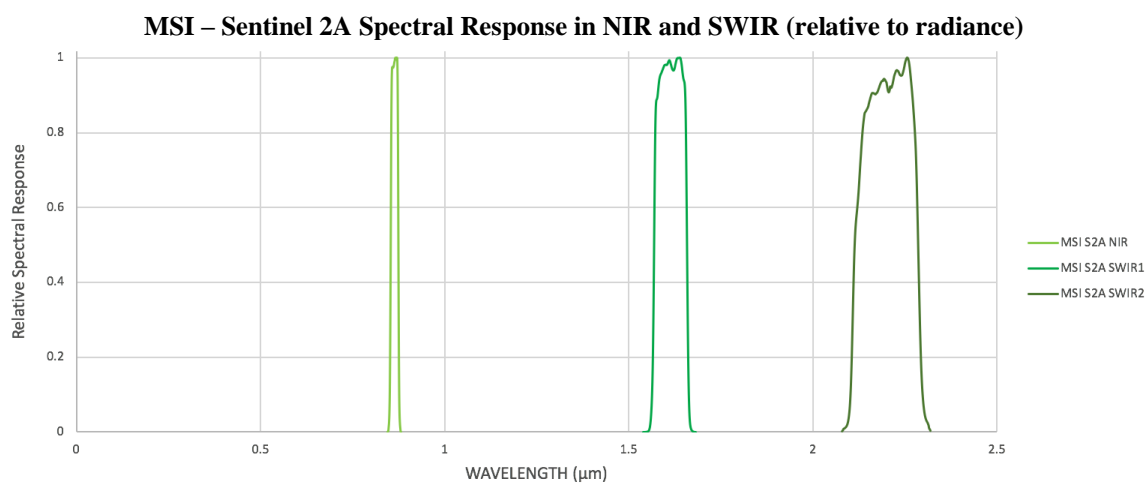
Figure 3.2 MSI for Sentinel 2A spectral response in NIR (0.85-0.88 \mu\text{m} ) and SWIR (1.53-1.68 \mu\text{m} and 2.08-2.32 \mu\text{m} respectively).
