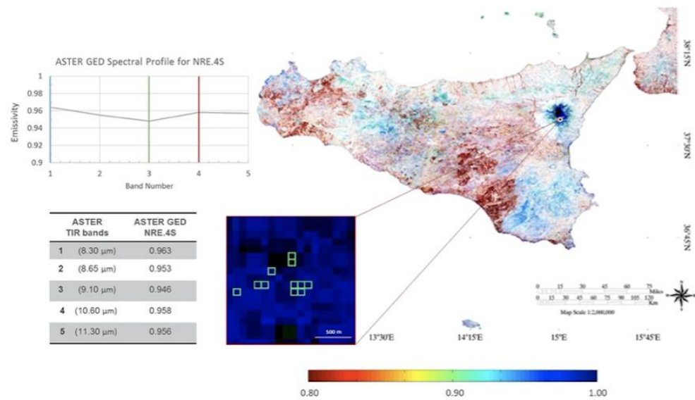
Figure 4. (Map) ASTER Global Emissivity Database (ASTER GED) over Sicily, Italy at 100-m pixel resolution at 10.60 μm and 4-3-1 band red-green-blue (RGB) view. The color ramp indicates the mean emissivity values (0.8–1.0). Inset shows samples' pixel locations for NRE.4S. Emissivity spectral profile plot and the table show emissivity variation with wavelength, extracted from ASTER GED for NRE.4S.
