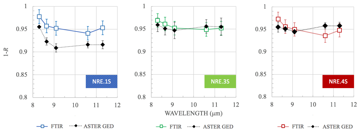
Figure 2.13 Comparison of reflectance FTIR derived ‘apparent’ emissivity results at 294 K (empty squares) with the spaceborne ASTER GED emissivity results for the same target area (black diamonds). A direct data comparison was made at five ASTER TIR bands.
