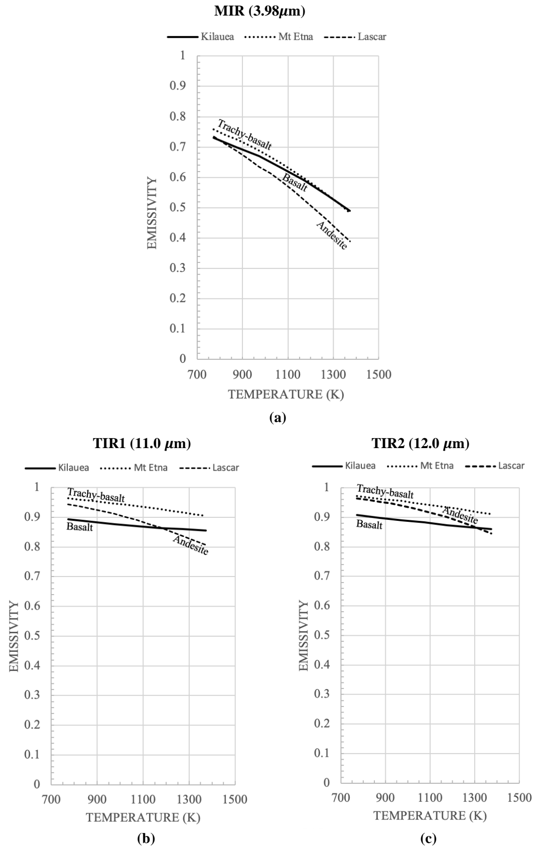
Figure 5.7 Trends diversity in MODIS' (a) MIR (3.98 \mu\text{m} ) and (b-c) TIR bands (11.0 \mu\text{m} and 12.0 \mu\text{m} respectively). Distinct compositional trends can be identified for trachy-basalt (Mt Etna), andesite (Lascar) and basalt (Kilauea).
