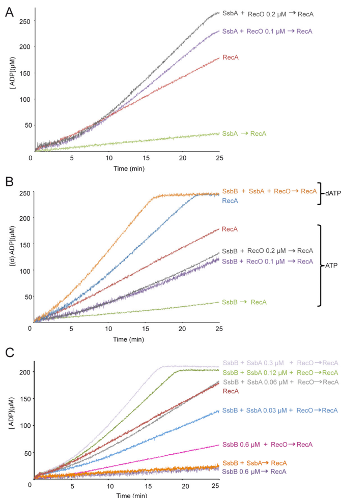
Figure 3. RecO facilitates RecA assembly on SsbA- or SsbB-coated ssDNA. (A) Circular pGEM3 Zf (+) ssDNA (10 μM in nt) was pre-incubated with SsbA (0.3 μM) or SsbB and RecO for 5 min at 37°C in buffer A containing 5 mM ATP. Then RecA (0.8 μM) was added and the ATPase activity measured for 25 min. (B) Circular ssDNA was pre-incubated with SsbB (0.3 μM) (or both SsbA [0.3 μM] and SsbB [0.3 μM]) and when indicated with RecO (0.1 and 0.2 μM) for 5 min at 37°C in buffer A containing 5 mM ATP or dATP. Then RecA (0.8 μM) was added and the (d)ATPase activity measured for 25 min. (C) The circular ssDNA was pre-incubated with a fixed amount of SsbB (0.6 μM), SsbA (0.3 μM) plus SsbB (0.3 μM) or a fixed amount of SsbB (0.3 μM) and increasing SsbA (0.03 to 0.3 μM) concentrations for 5 min at 37°C in buffer A containing 5 mM ATP. Then RecO (0.1 μM) was added to the preformed SSB-ssDNA complexes and incubated for 5 min at 37°C. Finally RecA (0.8 μM) was added and the ATPase activity measured for 25 min. All reactions were repeated three or more times with similar results.
