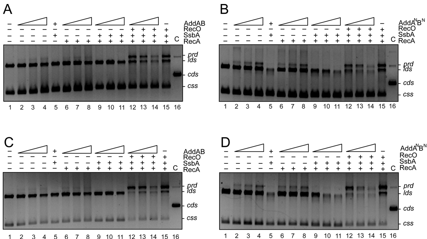
Figure 5. AddAB does not contribute to RecA-ATP activation to catalyze DNA recombination. Circular pGEMχ10F or pGEMχ10R ssDNA (10 μM in nt) and linear pGEMχ10F (χ10F, A and B) or pGEMχ10R (χ10R, C and D) dsDNA (20 μM in nt) were incubated with increasing AddAB or AddA N AddB N (0.35, 0.75 and 1.5 nM) concentrations for 60 min at 37°C in buffer A containing 5 mM ATP. The circular ssDNA and linear dsDNA substrate were pre-incubated with increasing AddAB or AddA N AddB N in the presence or absence of SsbA (0.3 μM) for 5 min at 37°C in buffer A containing 5 mM ATP. Then RecA (1.2 μM) was added and the reactions were incubated for 60 min at 37°C. In reactions where RecO was also added, the circular ssDNA and linear dsDNA substrate were pre-incubated with SsbA (0.3 μM), RecO (0.2 μM) and increasing AddAB or AddA N AddB N for 5 min at 37°C in buffer A containing 5 mM ATP. Then RecA (1.2 μM) was added and the reactions were incubated for 60 min at 37°C. The separation of the products and the symbols are the same as those described in Figure 4. The results are representative of more than three independent experiments.
