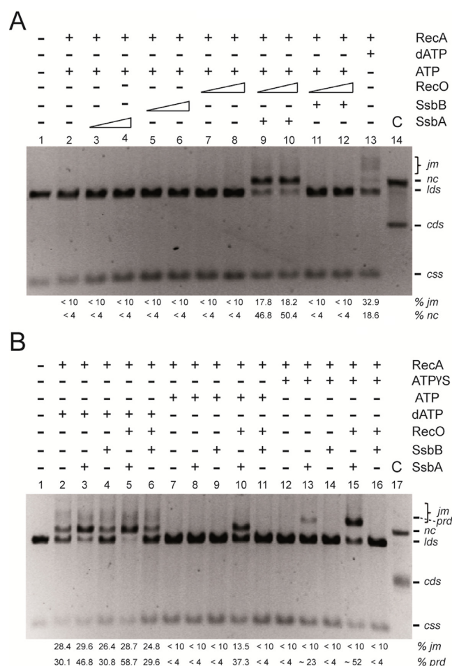
Figure 4. SsbA and RecO contribute to RecA-promoted DNA strand exchange. (A) Circular pGEM3 Zf (+) ssDNA (10 μM in nt) and homologous linear dsDNA (20 μM in nt) were pre-incubated with increasing concentrations of SsbA or SsbB (0.15 and 0.3 μM) or RecO (0.2 and 0.4 μM) for 5 min at 37°C in buffer A containing 5 mM ATP or dATP. In the indicated reactions, RecO (0.2 and 0.4 μM) was added to the preformed SsbA-ssDNA or SsbB-ssDNA (SSB 0.3 μM) complexes and incubated for 5 min at 37°C. Finally, RecA (1.2 μM) was added and the reaction was incubated for 60 min at 37°C. (B) The circular ssDNA and homologous linear dsDNA were pre-incubated with SsbA or SsbB (0.3 μM) for 5 min at 37°C in buffer A containing 5 mM dATP, ATP or ATPγS, and RecO (0.2 μM) was added to the preformed SsbA-ssDNA or SsbB-ssDNA complexes and incubated for 10 min at 37°C. Finally, RecA (1.2 μM) was added and the reaction was incubated for 60 min at 37°C. The products of the reactions were deproteinized, separated on a 0.8% AGE with ethidium bromide and quantified as described in 'Materials and Methods' section. The positions of the bands corresponding to css , cds , lds , jm , nc and ATPγS-generated prd products are indicated. Symbols + and - denote the presence or absence, respectively, of the indicated protein. In A (lane 14) and in B (lane 17) nicked circular pGEM3 Zf (+) plasmid DNA was added as a mobility control (C). The amounts of jms and products ( nc and prd ) are indicated and expressed as the percentage of total substrate added. The results are the average value obtained from more than three independent experiments (the results given stand within a 5% standard error).
