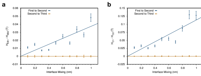
FIG. 10. The change in exchange bias and coercivity between the first and second and second and third simulated hysteresis loops (a) The change in the exchange bias between consecutive hysteresis loops, with lines of best fit to guide the eye. (b) The change in the coercivity between consecutive hysteresis loops, with lines of best fit to guide the eye. There is a large change in both the coercivity and the exchange bias between the first and second simulated hysteresis loops but almost no change between the second and third.
