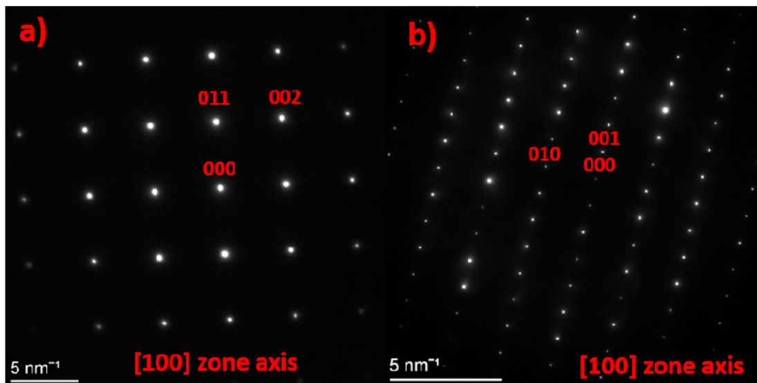
Fig. 9. SADPs from Si 0.1 TiVCr 0.5 after solution annealing of the a) BCC phase and b) Laves phase.
