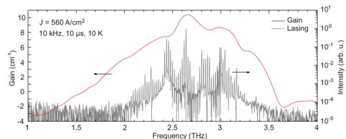
Figure 1: Comparison of the intensity gain, measured by THz time-domain spectroscopy in a coupled cavity configuration, and the lasing spectrum (FTIR) of an ultra-broadband THz QCL.
