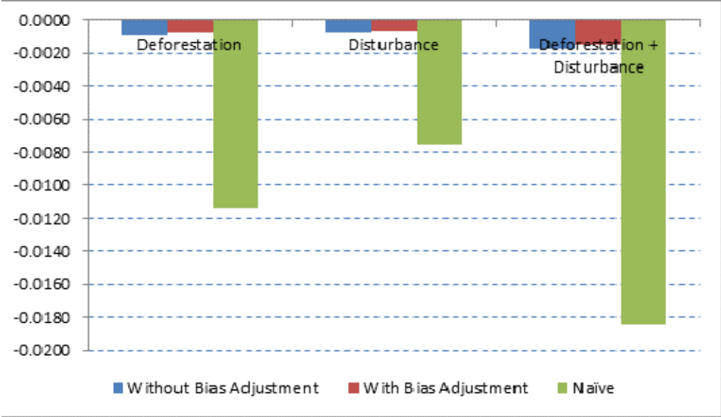
Figure 2 Forest cover change: Naïve effects and ATT
