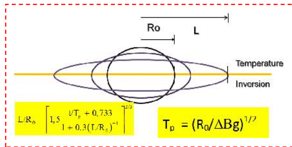
Fig. 5 Gravitational deformation from R_o to L in the time t with time constant T_p , relative density difference of ambient air layers is \Delta , and correction factor B . The g is the acceleration of gravity.
