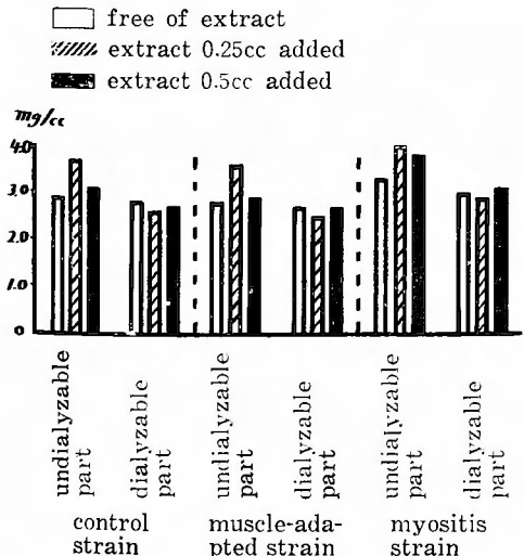
Fig. 8. Undialyzability of the factors comprised in the extract of skeletal muscles, influencing the growth of the staphylococci.
