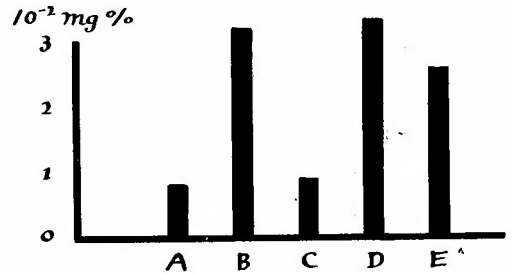
Fig. 19. Effect of the extracts of skeletal muscles and bone-marrow on staphylococcal lecithinase activity.
