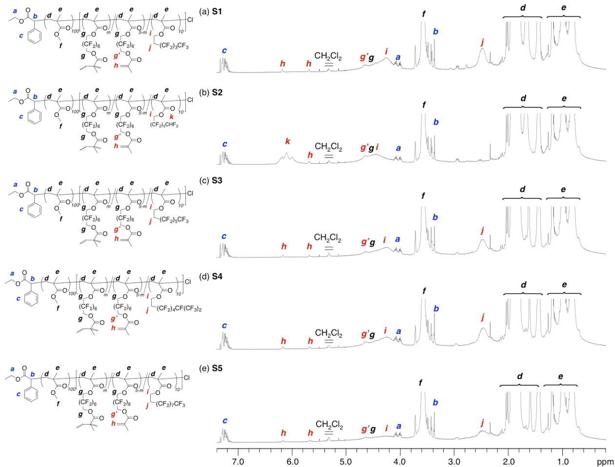
Figure 2. ^1\text{H} NMR (500 MHz) spectra of (a) S1, (b) S2, (c) S3, (d) S4, and (e) S5 ([star] = 50 mg/mL) in \text{CD}_2\text{Cl}_2 at 30^\circ\text{C} .
