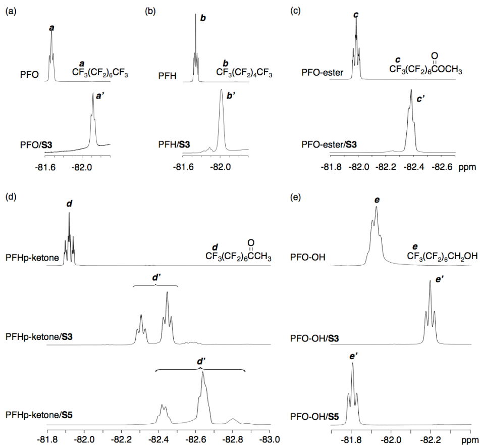
Figure 7. ^{19}\text{F} NMR (470 MHz) spectra of polyfluorinated guests (a: PFO, b: PFH, c: PFO-ester, d: PFHp-ketone, e: PFO-OH) with S3 or S5: [S3 or S5] = 50 mg/mL in \text{DMF-}d_7 at 30 °C.
