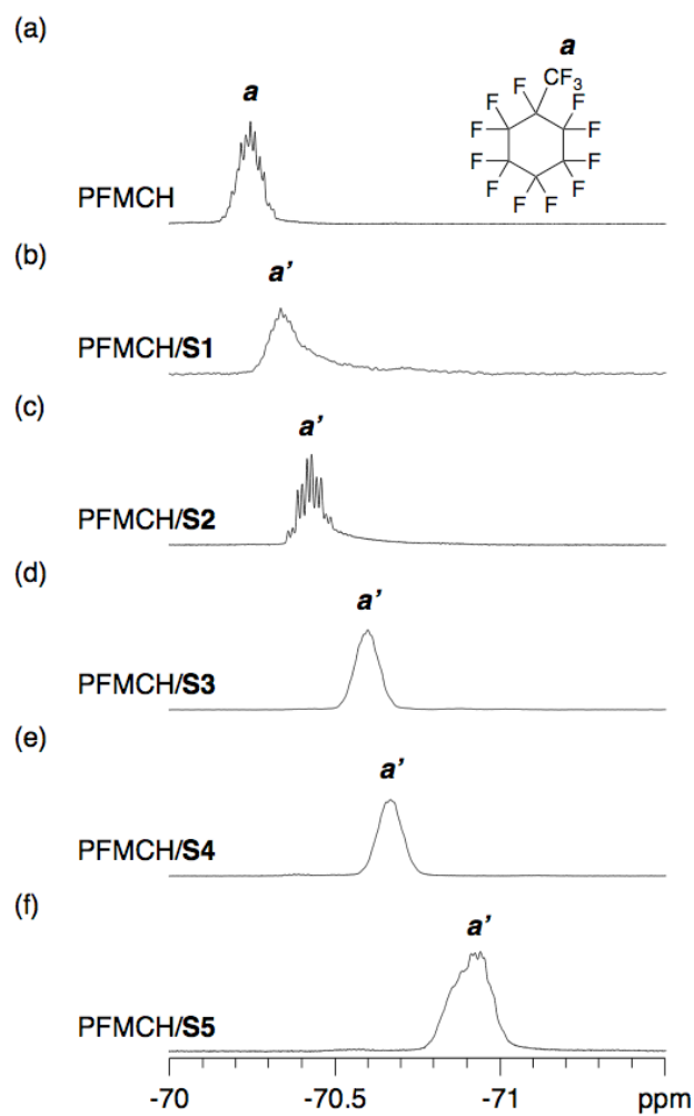
Figure 5. ^{19}\text{F} NMR (470 MHz) spectra of (a) PFMCH alone and (b-f) PFMCH with S1-S5 (b: S1, c: S2, d: S3, e: S4, f: S5): [S1-S5] = 50 mg/mL in \text{DMF-}d_7 at 30 °C.
