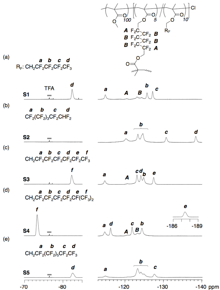
Figure 3. ^{19}\text{F} NMR (470 MHz) spectra of (a) S1 , (b) S2 , (c) S3 , (d) S4 , and (e) S5 ([star] = 50 mg/mL) in \text{CDCl}_3 at 30 °C (TFA: trifluoroacetic acid, \delta = -76.5 ppm).
