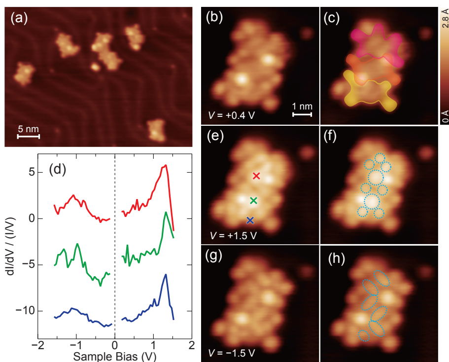
Fig. 5 (a) Typical STM images of zinc porphyrin array [(\text{ZnP})_3] on Au(111) ( V = +0.4 V and I = 50 pA). (b) A close-up view of a porphyrin array. (c) The same as (b) superimposed by schematic illustration of each component. (d) Normalized dI/dV curves of the array (offset for clarity). The red, green, and blue curves are recorded over the position marked by the crosses of corresponding colors in (e). The STM images of a (\text{ZnP})_3 molecule acquired with (e) V = 1.5 V and (g) V = -1.5 V at I = 50 pA. The bias-dependent STM images in (e) and (g) show unoccupied orbitals and occupied orbitals, respectively. The images (f) and (h) are the same as (e) and (g), respectively, but superimposed by the ellipses illustrating the shape of the orbitals distributed in each macrocycle.
