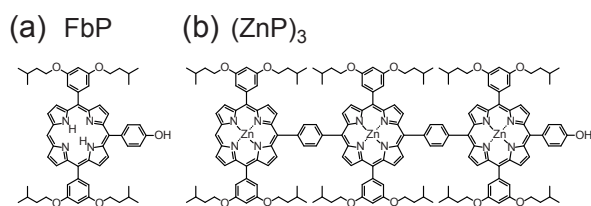
Fig. 1 Molecular structures of (a) freebase porphyrin monomer (FbP) and (b) phenylene-linked Zn porphyrin array [(ZnP) 3 ].
