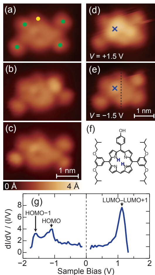
Fig. 3 (a)–(c) Sequential STM images of an isolated FbP molecule ( V = +0.4 V and I = 50 pA). The yellow and green dots in (a) indicate the hydroxyphenyl and isoamyloxy groups, respectively. The appearance and position of the dots change between sequential imaging, which is caused by the inevitable perturbation by the tip. (d), (e) STM images of FbP acquired with V = (d) +1.5 V and (e) -1.5 V at I = 50 pA. The porphyrin core appears asymmetric with respect to the molecular axis (dashed line). (f) Schematic illustration of the molecular structure of an FbP molecule. (g) A normalized dI/dV spectrum of the FbP molecule recorded over the cross in (e). The black arrows represent resonance peaks of the molecular orbitals.
