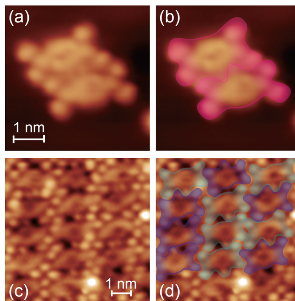
Fig. 4 (a) The STM images of dimerized FbP molecules ( V = +0.4 V and I = 50 pA). (b) The same as (a) superimposed by the envelopes representing the contour of the molecules (head-to-head configuration). (c) The STM images of the monolayer FbP ( V = +0.4 V and I = 50 pA). (d) The same as (b) superimposed by the envelopes representing the contour of the molecules. Blue and cyan envelopes represent the molecules which are rotated by 180^\circ with each other.
