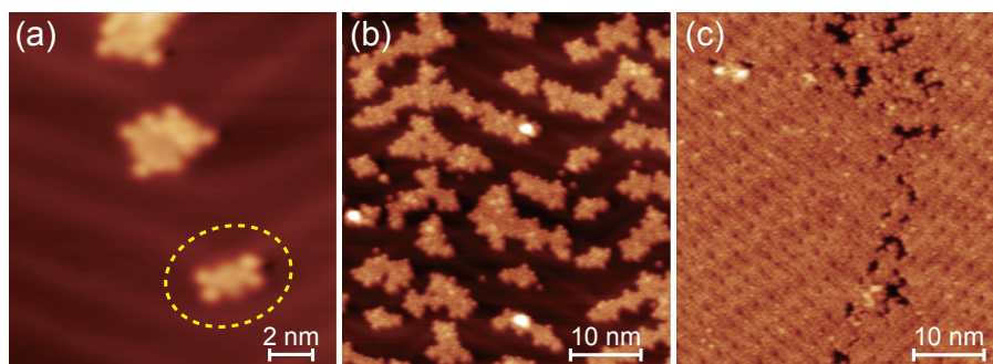
Fig. 2 (a)–(c) Typical STM images of freebase porphyrin monomers (FbP) on Au(111) as a function of the coverage. The molecules were adsorbed on the surface at \sim 90 K, and the images were obtained at 6 K in the constant-current mode with a sample bias V = +0.4 V and tunnel current I = 50 pA. An isolated molecule (surrounded by a dotted ellipse) is observed at low coverage in (a), and then, the clusters and monolayer develop as the coverage increases as shown in (b) and (c), respectively.
