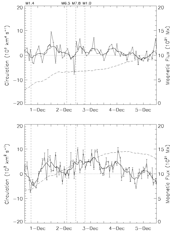
Figure 11. Time variations of circulation (thin solid lines) and magnetic flux (dashed lines) in sunspots n1 (top) and p2 (bottom) in NOAA 10826. The format is the same as in Figure 7.
