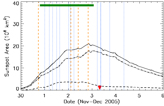
Figure 12. Time evolution of umbra (dashed), penumbra (dash-dotted), and total sunspot (solid) areas in NOAA 10826. The format is the same as in Figure 8.
