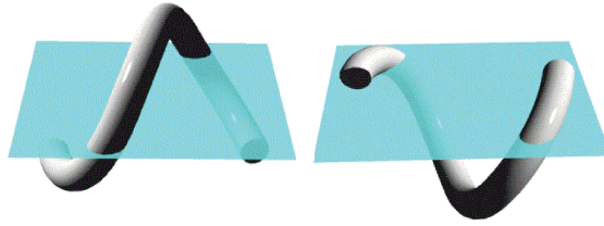
Figure 3. Illustrations of the emergence of tubes with left-handed writhe in the cases of upward-kinked and downward-kinked configurations. In both cases, the inclination angle of the line connecting the two footpoints rotates clockwise and their separation increases or decreases according to the orientation of the kink.
