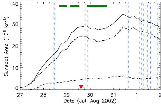
Figure 16. Time evolution of umbra (dashed), penumbra (dash-dotted), and total sunspot (solid) areas in NOAA 10050. The format is the same as in Figure 8.
