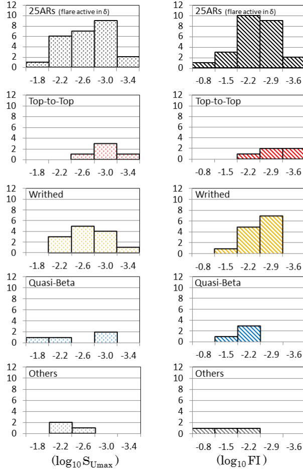
Figure 19. Histograms of umbral area maximum (left) and FI (right) in the \delta -state period. From the second row downward are shown “top-to-top”, “writhed”, “quasi- \beta ”, and “others” types, respectively, and the top row shows the total.
