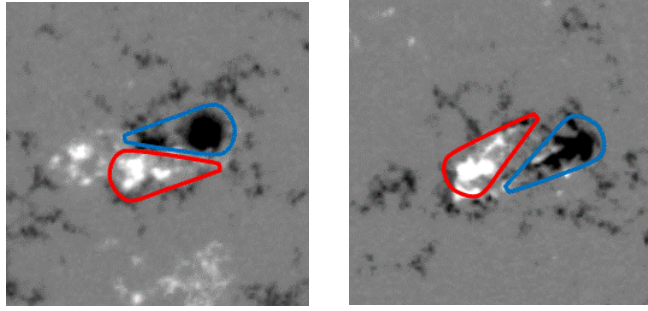
Figure 4. Sample images of magnetic tongues. When the head parts of the “Yin-Yang” structure forming the magnetic tongues show clockwise or counter-clockwise orientation, they indicate negative or positive magnetic helicity, respectively.
