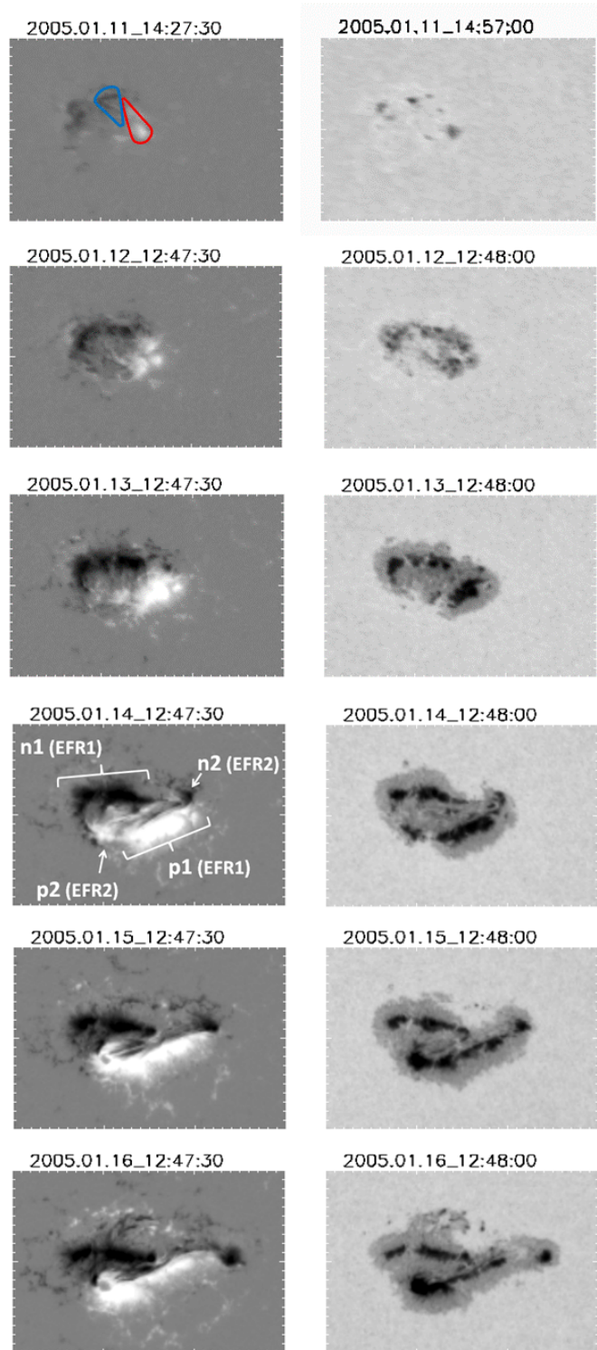
Figure 5. SOHO/MDI magnetograms (left) and white-light images (right) of NOAA 10720 corresponding to subsequent days of observations. Identified two EFRs are shown in the fourth row. The field of view (FOV) of each panel is 300 \times 200 arcsec.
