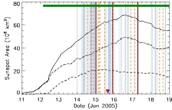
Figure 8. Time evolution of umbra (dashed), penumbra (dash-dotted), and total sunspot (solid) areas in NOAA 10720. Vertical lines indicate X-class (brown solid), M-class (orange dashed), and C-class (blue dotted) flares, respectively. The horizontal thick green line at the top represents the duration of the \delta -state. The triangle at the bottom indicates the central meridian passage of the region.
