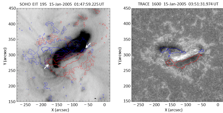
Figure 9. Left: A SOHO/EIT 195Å image (in negative print) of NOAA 10720 taken at 01:47 UT, 15 January 2005, after the X1.2 flare peaked at 01:02 UT. White arrows indicate two polarities of EFR2. An inverse-S shaped structure is clearly seen. Right: A TRACE 1600Å image taken at 03:51 UT on 15 January 2005 between the two X-class flares. A bright structure existed between the two polarities of EFR2 even in a relatively quiet period of flare activity. Overlaid contours (red for positive and blue for negative polarities) show the line-of-sight magnetic fields of 1500 gauss (G) and 100 G (only in the left panel). The FOV of both images is 300 \times 300 arcsec.
