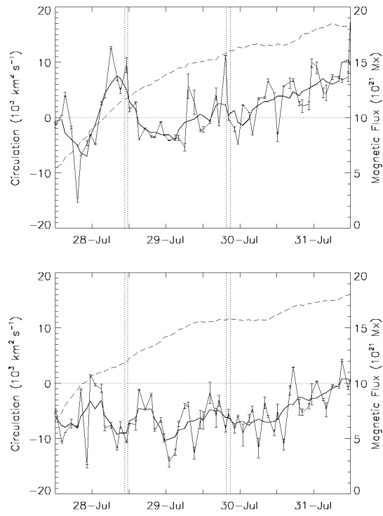
Figure 15. Time variations of circulation (thin solid lines) and magnetic flux (dashed lines) in the preceding negative polarity sunspot (top) and the following positive polarity sunspot (bottom) in NOAA 10050. The format is the same as in Figure 11. Dotted vertical lines represent C-class flares.
