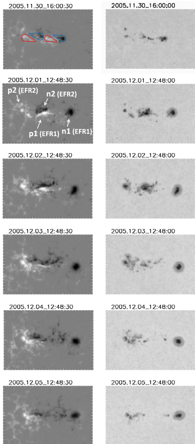
Figure 10. SOHO/MDI magnetograms (left) and white-light images (right) of NOAA 10826. Identified two EFRs are shown in the second row. The FOV of each panel is 300 \times 200 arcsec.
