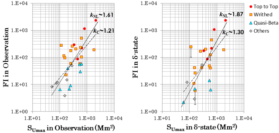
Figure 18. Flare index versus maximum umbral area in a logarithmic scale. The left panel is for the data in the observed period and the right panel is for those in the \delta -state. Six ARs which showed no flare activity in the \delta -state were excluded. Different symbols indicate “top-to-top” (red circles), “writhed” (orange squares, both DK and UK types in Table 1), “quasi- \beta ” (blue triangles), and “others” (gray diamonds), respectively. The error-bars were assigned by considering the effect of data gaps (see text). The results of non-linear least-squares fitting (power-law index k_{NL} ) and classical least-squares fitting (power-law index k_C ) are shown by the solid and the dashed lines, respectively.
