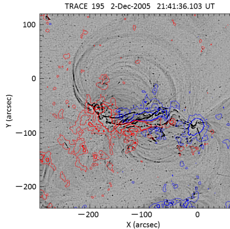
Figure 13. A high-pass filtered TRACE 195 Å image (in negative print) of NOAA 10826. Contours indicate line-of-sight magnetic fields of 500 G (thick) and 100 G (thin) in positive (red) and negative (blue) polarity areas. After the M1.0 flare, highly-sheared bright structures appeared on the \delta -part of the region.
