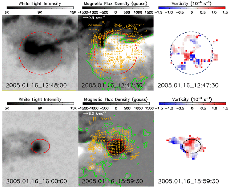
Figure 6. White light images (left), magnetograms (middle), and vorticity fields (right) of the positive (top row) and negative (bottom row) polarity areas of EFR2, respectively. The size of each FOV is 100 \times 100 arcsec, and its center is at the center of gravity of magnetic flux distribution. In the middle panels are overlaid the velocity fields (yellow arrows) and the neutral lines (green contours). The areas used to compute the circulation are shown by a circle of 28 arcsec radius in the top row and by an ellipse in the bottom row whose major and minor axes are 24 and 18 arcsec, respectively.
