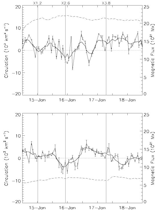
Figure 7. Time variations of circulation (thin solid lines) and magnetic flux (dashed lines) in sunspots p2 (top) and n2 (bottom) in NOAA 10720. The thick solid line shows the running average of circulation over five consecutive data points in each panel. The error bars indicate a possible range of the circulation values when the size of the analysis area is changes (see text). Vertical lines represent the times of the X-class flares. The magnetic flux values are evaluated for the full FOV of Figure 6.
