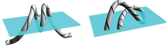
Figure 20. Schematic models for \beta\gamma\delta ARs. The left panel shows a general model for the downward-knotted type such as NOAA 10826. The right panel shows a possible model for the “top-to-top” type such as NOAA 10720.
