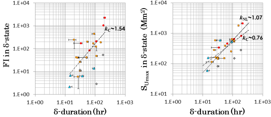
Figure 21. Flare Index (left) and maximum umbral area (right) in the \delta -state as a function of the \delta -duration. The symbols are the same as in Figure 18. Six ARs which showed no flare activity in the \delta -state were excluded. The error-bars were assigned by considering the effect of data gaps (see text). The results of non-linear least-squares fitting (power-law index k_{NL} ) and classical least-squares fitting (power-law index k_C ) are shown by the solid and the dashed lines, respectively.
