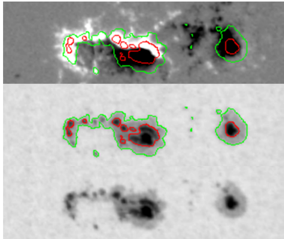
Figure 1. A magnetogram (top, gray scale) and a white light image (bottom) of NOAA 10314. Green and red contours show the intensity levels of 0.9 and 0.65 of the quiet region (QR) intensity and delineate QR-penumbra boundaries and penumbra-umbra boundaries, respectively (the middle panel). The AR has \delta -configuration in the central part.
