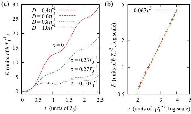
FIG. 2. (Color online) (a) Time dependence of the total energy E at n = 6 , r = 1 , u = 10\hbar T_0^{-1}\eta , v = 4\eta/T_0 for the four cases D = 0.4\eta^{-1} , D = 0.6\eta^{-1} , D = 0.8\eta^{-1} , and D = 1.0\eta^{-1} . (b) Trap speed dependence of total energy increase per unit time P at n = 1 , D = 0.5\eta^{-1} , r = 1 , u = 10\hbar T_0^{-1}\eta (log scale).
