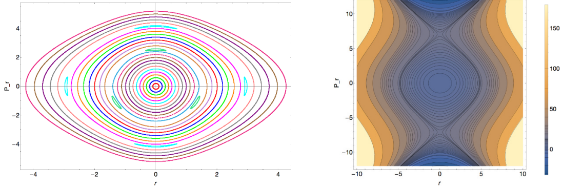
(a) Poincaré section with E = 10 .
