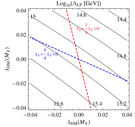
Fig. 1. A contour plot of the scale of the LP as functions of \lambda_X, \lambda'_X at \mu = M_X with M_X = 100 GeV. The red and blue lines represent to \lambda_X + 1/4\lambda'_X = 0 and \lambda_X + 9/4\lambda'_X = 0 , respectively. The left-bottom side of the red or blue line corresponds to the unbounded scalar potential.
