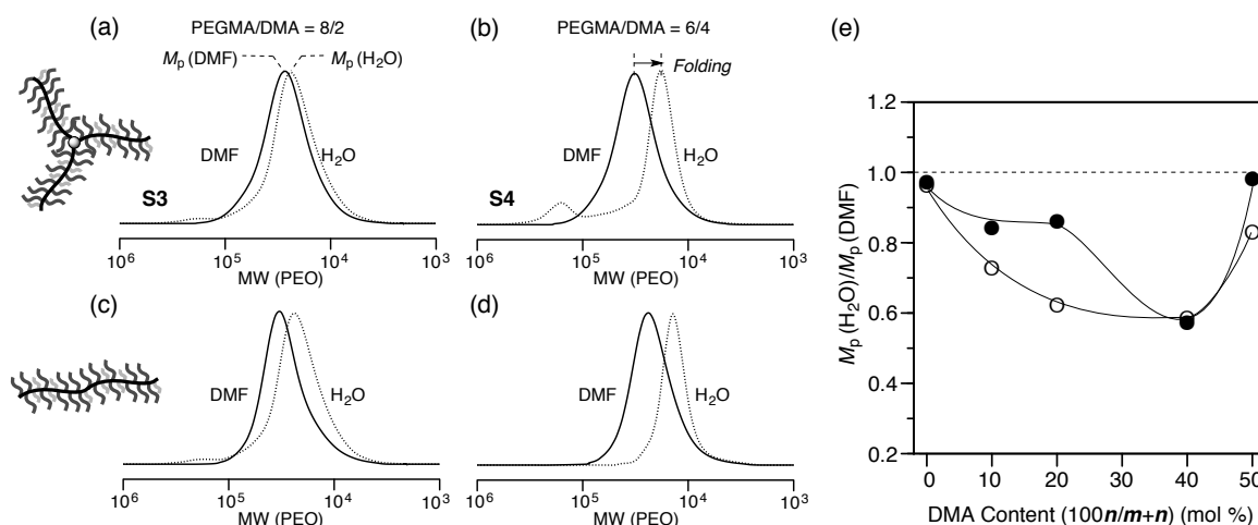
Figure 3. SEC curves in DMF or H 2 O for (a, b) 3-armed star PEGMA/DMA random copolymers (a: S3 , b: S4 ) and (c, d) linear PEGMA/DMA random copolymers (c: 160/40, d: 120/80). (e) SEC peak top molecular weight ratio [ M_p(H_2O)/M_p(DMF) ] for 3-armed star PEGMA/DMA random copolymers ( S1-S5 : filled circle) and linear PEGMA/DMA ( m/n ) random copolymers ( m/n = 200/0 - 100/100 : open circle).
