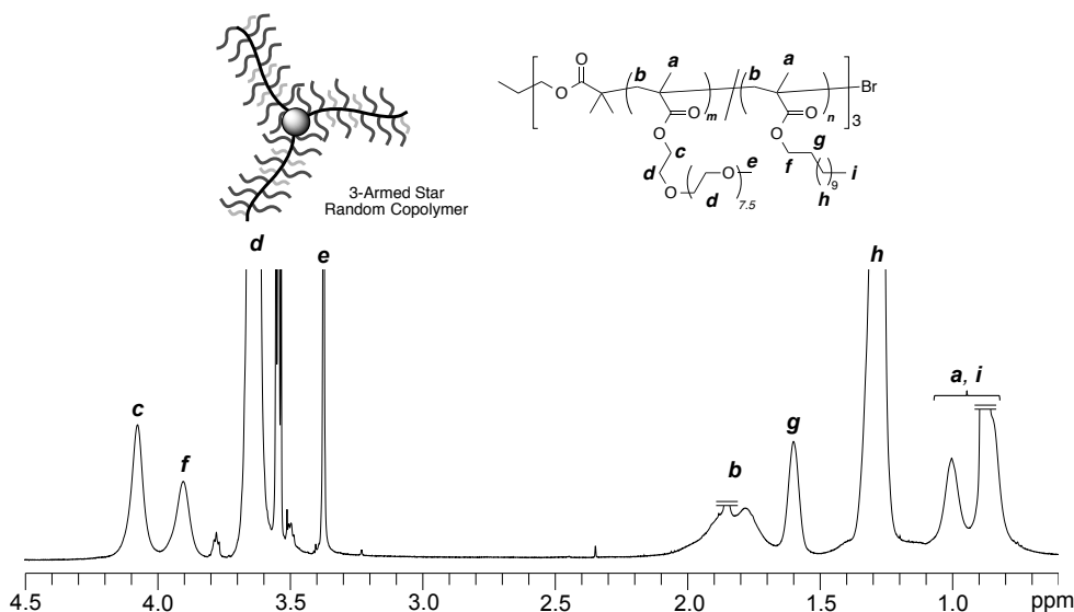
Figure 2. ^1\text{H} NMR spectrum of S4 ( m/n = 44/29 ) in \text{CHCl}_3 at 25\text{ }^\circ\text{C} .
