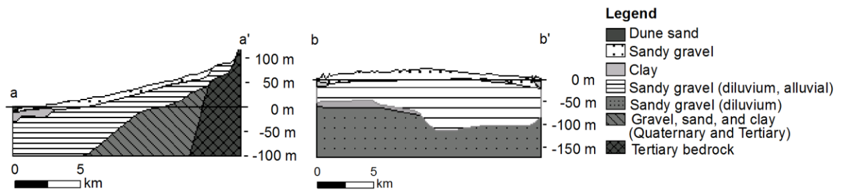
Fig. 2 Hydrogeological conditions across the study area (sections a-a' and b-b' in Fig.1) (Modified From Hokuriku Regional Agricultural Administration Office 1977)
