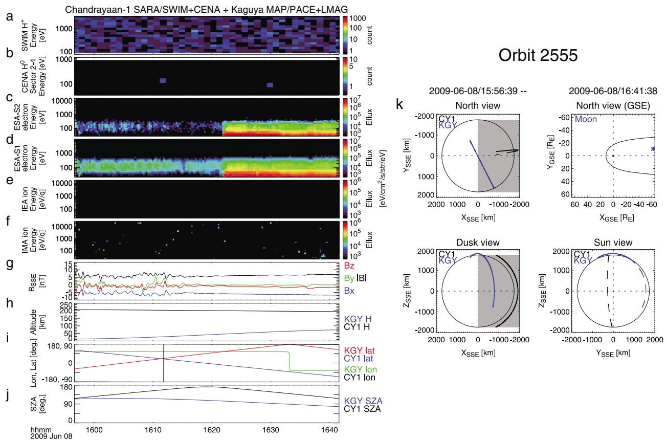
Figure 2. Time series data from Chandrayaan-1 (orbit 2555) and Kaguya in the terrestrial magnetotail in the same format as in Figure 1. Kaguya was illuminated by sunlight after 16:22 UT and intense spacecraft photoelectrons which were attracted by the positive spacecraft potential can be seen in the low-energy part of the (d) ESA-S1 and (c) ESA-S2 data. The fluctuations observed by (g) L2-MAG at 15:56–16:18 UT at low altitudes are presumably due to lunar crustal magnetic fields.
