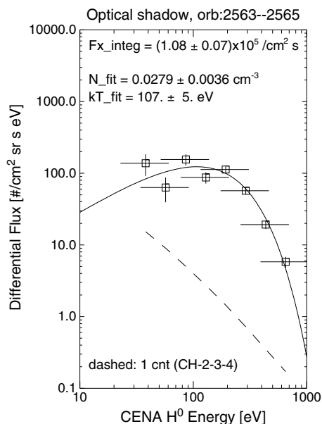
Figure 4. Energy spectrum of upward traveling hydrogen ENAs detected by CENA in the optical shadow of the Moon integrated over the orbits 2563–2565. Error bars correspond to the energy resolution (x axis) and the uncertainty due to counting statistics (y axis). The upward flux derived from the observed differential flux integrated over the measured energy range is shown with errors from propagation of counting statistics. The solid curve shows the best fitted Maxwell distribution. The fitting parameters with errors from propagation of the fitting errors are also denoted. The dashed line represents the one count level (over 135 min).
