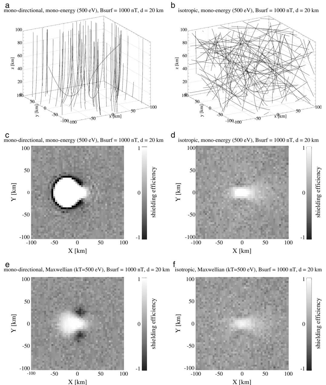
Figure 7. Test particle trajectories around a buried dipole using different proton velocity distributions. A part of proton trajectories for (a) monodirectional and (b) isotropic initial velocity distributions with a constant energy of 500 eV, in addition to the shielding efficiencies on the surface (see text for details) for (c) monodirectional and (d) isotropic monoenergy protons (500 eV) and (e) monodirectional and (f) isotropic Maxwellian protons ( kT = 500 eV) are shown. The dipole is horizontally placed along y axis. The dipole magnetic field has -y component above the surface.
