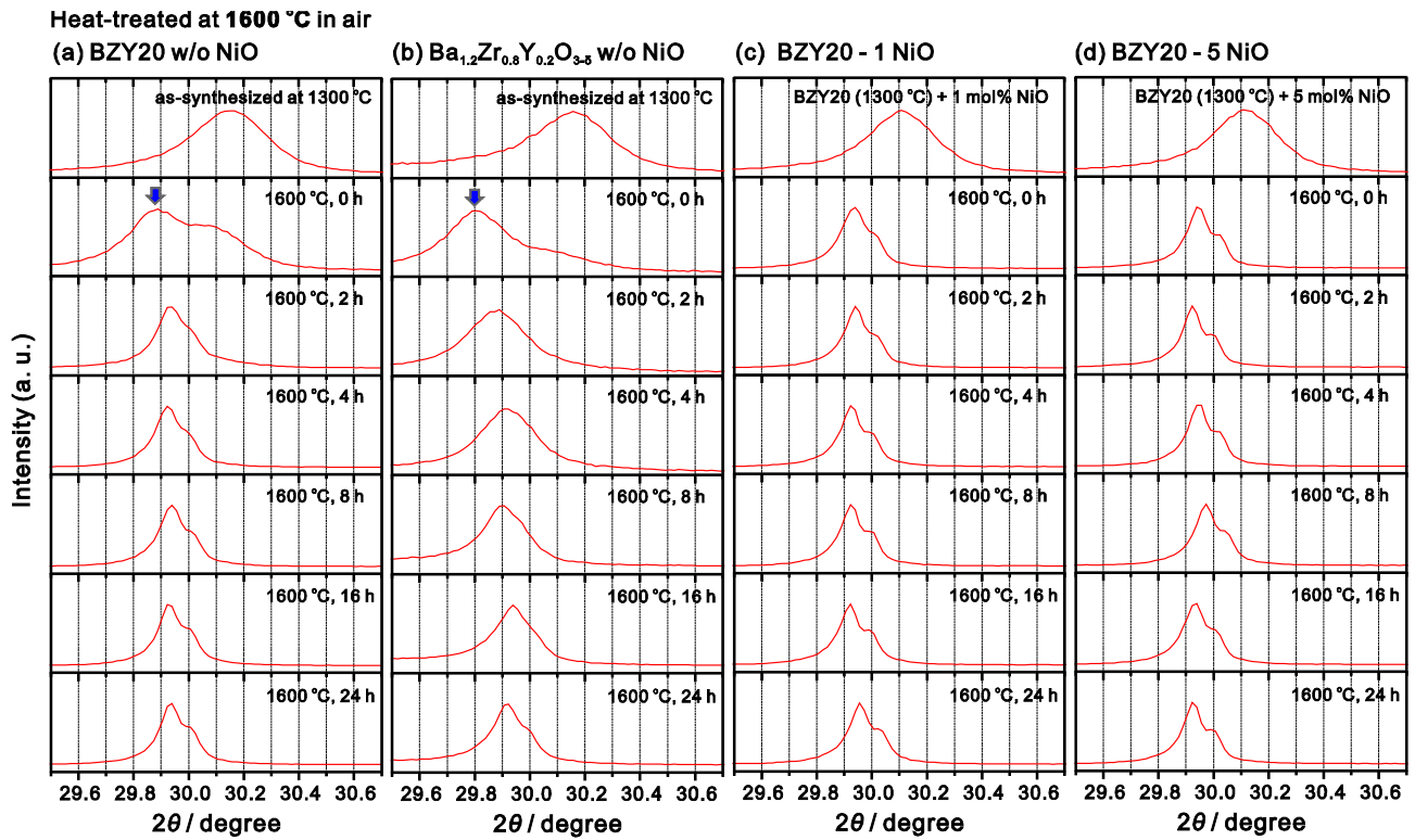
Fig. 8 Variation of (011) diffraction peak shape of (a) BZY20, (b) Ba_{1.2}Zr_{0.8}Y_{0.2}O_{3-\delta} , (c) BZY20 – 1 NiO, and (d) BZY20 – 5 NiO, which were heat-treated at 1600 °C in air for different time. The samples were finally quenched in ambient atmosphere.
