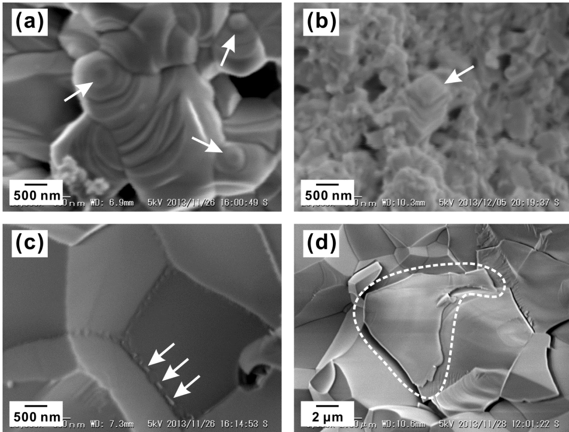
Fig. 5 SEM images of trace of liquid phase marked by arrows in Ba_{1.2}Zr_{0.8}Y_{0.2}O_{3-\delta} heat-treated at (a) 1600 °C, and (b) 1400 °C in air for 24 h, and (c) BZY20 – 1 NiO heat-treated at 1600 °C for 24 h, and highlighted by a dashed circle in (d) BZY20 – 5 NiO heat-treated at 1600 °C for 16 h. All the samples were finally quenched in ambient atmosphere.
