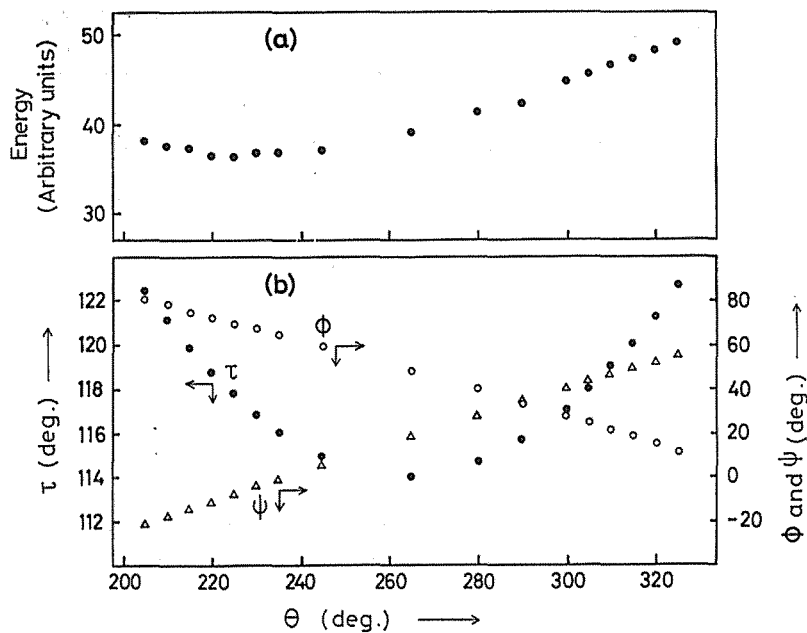
Fig. 8 Relationships between virtual bond rotation and conformational energy (a), and the resulting \tau , \phi and \psi angles (b) for a left-handed CTP, where O ( \circ ) is gt, and CM ( \triangle ) is trans positions.
