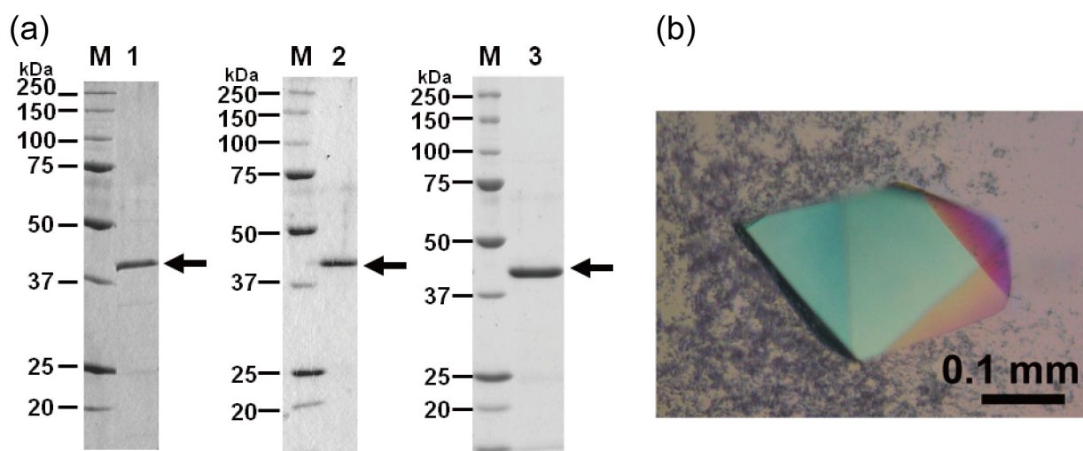
Figure 1-3. Purification and crystallization of streptococcal UGLs. (a) SDS-PAGE profile. Lane M, molecular weight standards (from top): synthetic polypeptides with molecular weights of 250,000, 150,000, 100,000, 75,000, 50,000, 37,000, 25,000, and 20,000; lane 1, SagUGL; lane 2, SpnUGL; lane 3, SpyUGL. (b) SagUGL crystal.
