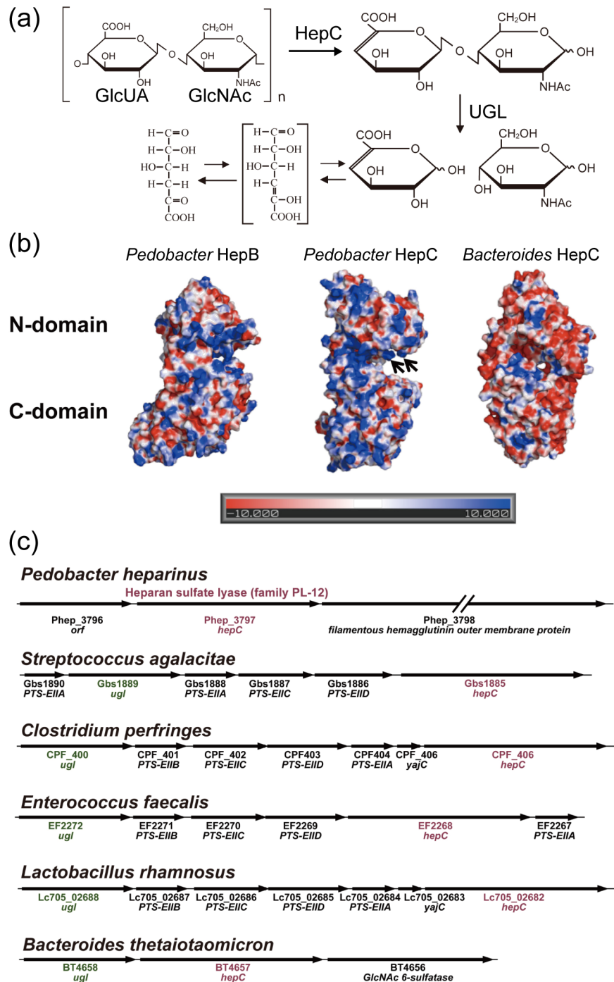
Figure 3-1-1. Heparin lyases. (a) Scheme for heparan sulfate degradation by HepC. Heparan sulfate includes sulfate group-free GlcUA-GlcNAc as a major disaccharide-repeating unit. (b) Electrostatic features on molecular surface model. Left , Pedobacter HepB; center , Pedobacter HepC; and right , Bacteroides HepC. Positive and negative charges are colored blue and red, respectively. Positively charged clusters at the active cleft of Pedobacter HepC are indicated by arrows . (c) Bacterial UGL gene clusters. PTS-EIIA–D: subunit domains of a phosphotransferase system for amino sugar import.
