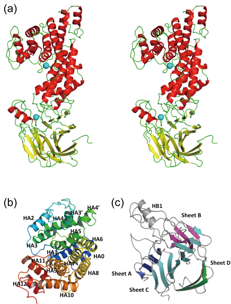
Figure 3-1-3. Structure of Pedobacter HepC. (a) Overall structure (stereo-diagram) (ball colored cyan: calcium ion). Colors denote secondary structure elements (red: \alpha -helices; yellow: \beta -strands; green: loops and coils). (b) N-terminal \alpha/\alpha -barrel composed of twelve \alpha -helices. (c) C-terminal antiparallel \beta -sheets (Sheets A–D).
