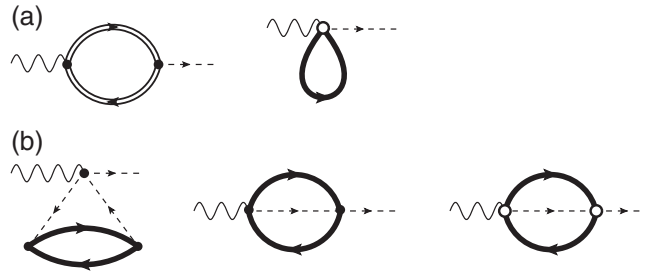
Fig. 4. Feynman diagrams showing the one-particle vertex correction of the pion decay constant \hat{f}_\pi . (a) Leading order density corrections. (b) Next-to-leading order corrections. In these diagrams, the wavy line denotes the axial vector current.
