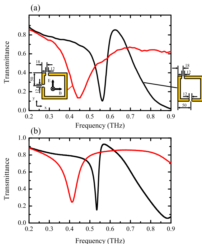
FIG. 6. (a) Measured and (b) simulated transmission spectra for double-gap SRRs of different geometrical parameters at normal incidence. Insets of (a) show the geometrical parameters of the SRRs.
