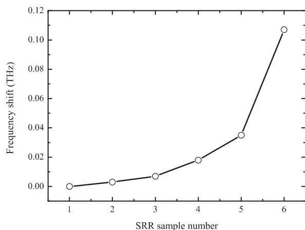
FIG. 5. Shift of resonant frequency between our original SRRs shown in Fig. 1 (SRR1-SRR6) and SRRs that consist of only longer metallic segment of each original SRR as a function of number of SRRs.
