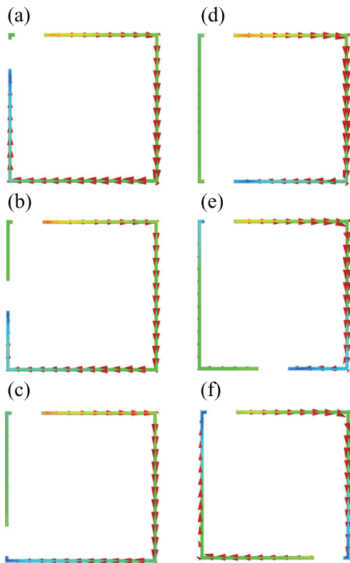
FIG. 3. Simulated distributions of surface current flow (arrow) and electric charge (color image) for SRR1-SRR6 at each resonant frequency. All figures are depicted at same phase for each resonant frequency (enhanced online) [URL: http://dx.doi.org/10.1063/1.4739945.1 ] [URL: http://dx.doi.org/10.1063/1.4739945.2 ] [URL: http://dx.doi.org/10.1063/1.4739945.3 ] [URL: http://dx.doi.org/10.1063/1.4739945.4 ] [URL: http://dx.doi.org/10.1063/1.4739945.5 ] [URL: http://dx.doi.org/10.1063/1.4739945.6 ].
