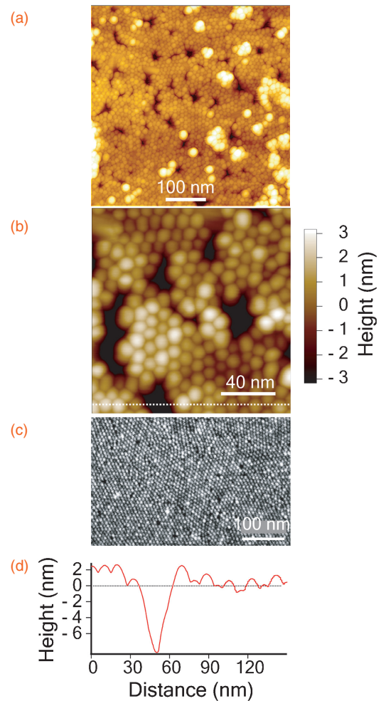
Fig. 3. (a) AFM image of dodecanethiol-coated 10 nm AuNP 2D array on the sputtered ITO (10.7 nm)/quartz (0.625 mm) substrate, (b) its magnification, and (c) corresponding SEM image. (d) Height profile along the white dotted line in (b).
