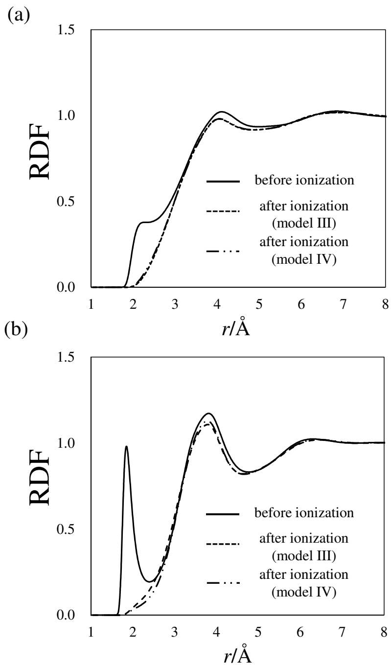
Figure 2: RDFs between (a) C_6 and H_w , (b) N_7 and H_w .
