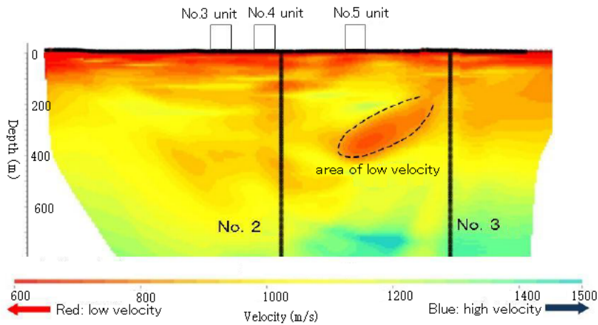
Fig.2(b) Deep ground profile
