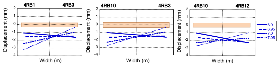
Deformation of No.4 unit foundation
