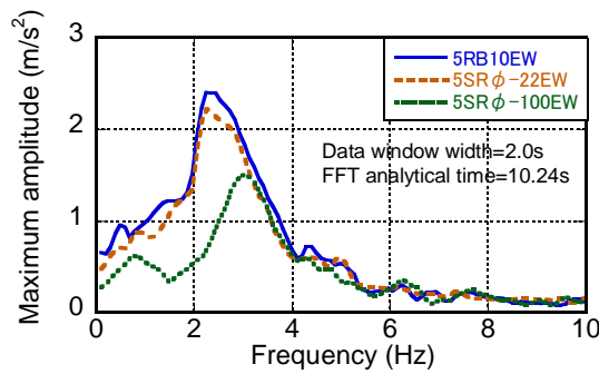
Fig.9 Non-stationary Fourier spectra (top) and maximum amplitude spectra (bottom) beneath the center of reactor building
