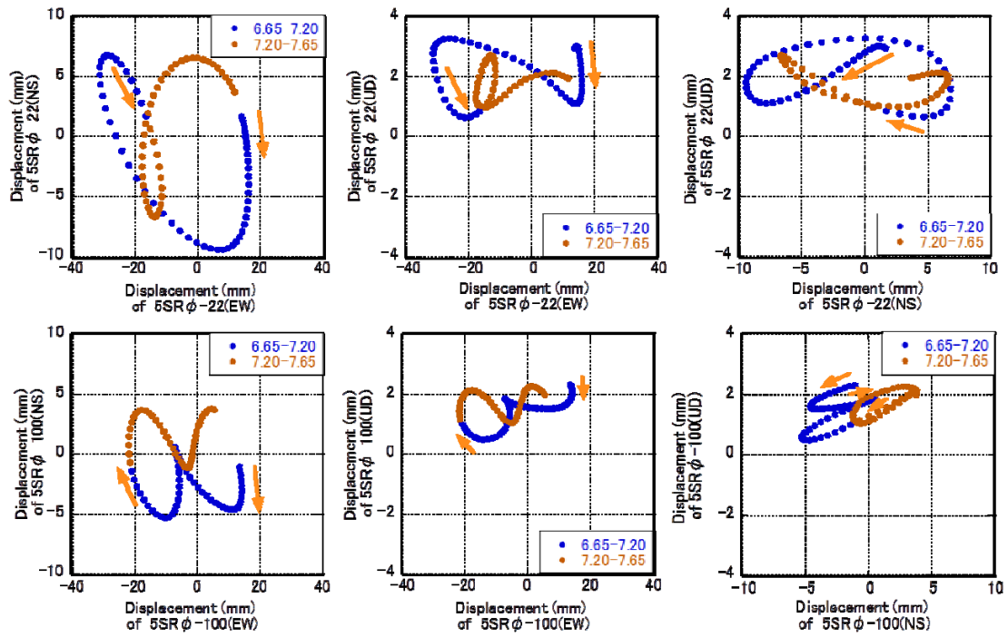
Fig.35 Orbit of displacement
