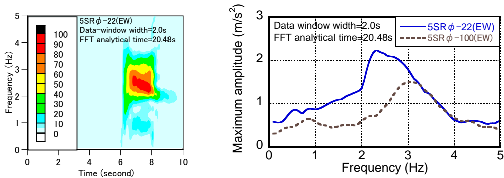
Fig.21 Non-stationary Fourier spectra and maximum amplitude spectra beneath the center of reactor building at No.5 unit (GL-22m)
