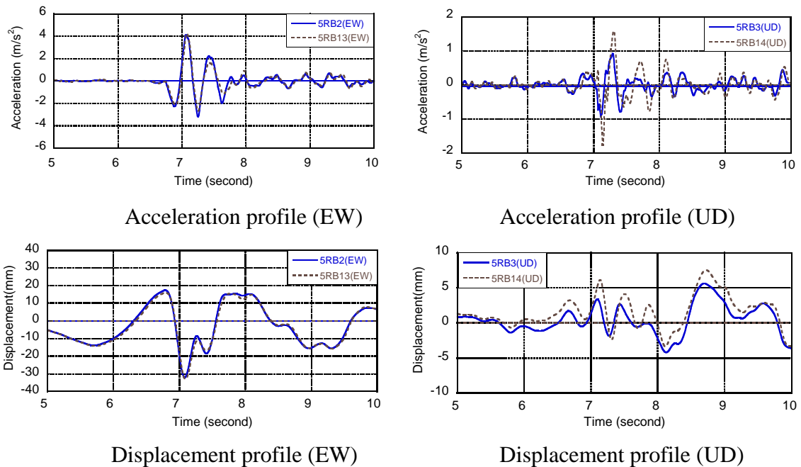
Fig.23 Acceleration and displacement profiles (No.5 unit)
