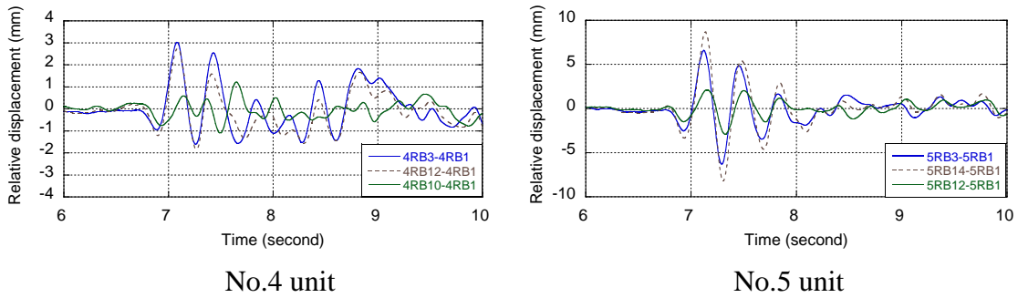
Fig. 29 Deformation of foundation
