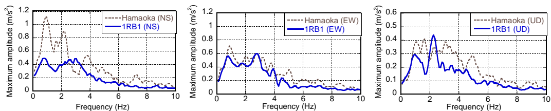
Fig.A2-2 Comparison of maximum amplitude spectra at K-NET (Hamaoka) and 1RB1
