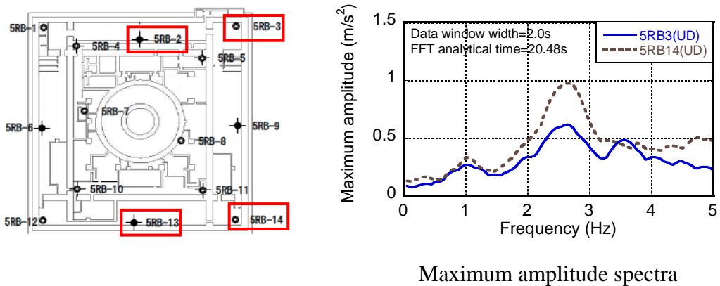
Fig.24 UD component on foundation at reactor building (No.5 unit)
