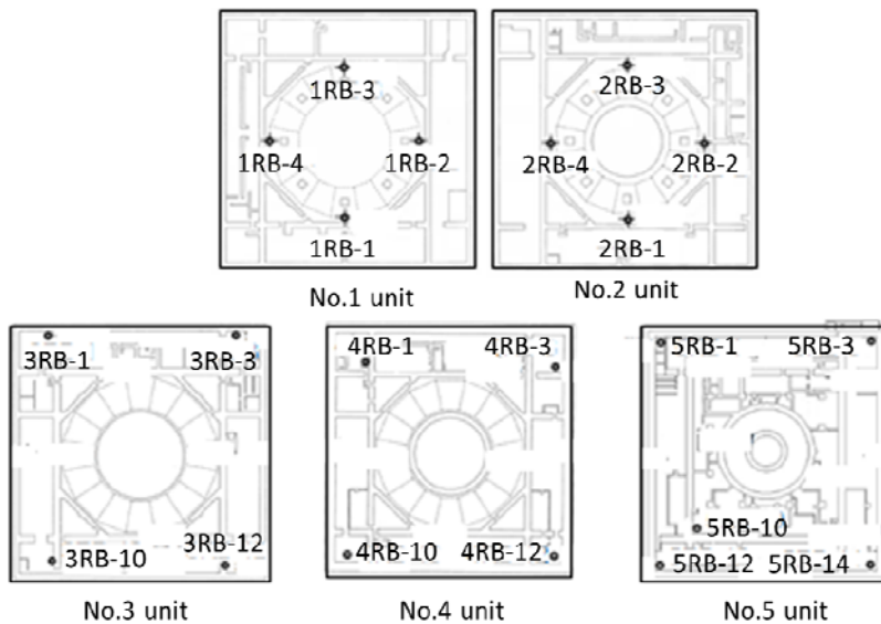
Fig.3 Arrangement of accelerometers in reactor buildings (RB: BF2-floor)
