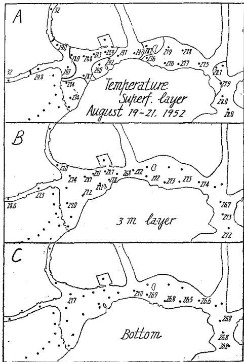
Fig. 5. Distribution of water temperature (°C) during August 19-21, 1952.
