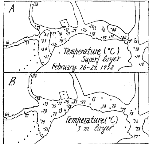
Fig. 3. Distribution of water temperature (°C) during February 26-27, 1952.
