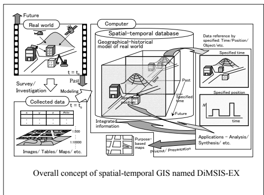
Fig. 8 Concept of Spatial-Temporal Database
