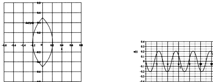
Figure 3.1: (left):The phase portrait of the \omega(= \pi) -periodic solution in the initial condition: u(0) = 0, \dot{u}(0) = -\frac{1}{2} in Example 3.1. (right): The time history of the \omega(= \pi) -periodic solution. The time is shown up to four periods.
