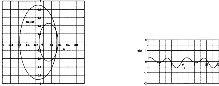
Figure 3.5: (left):The \omega(= 2\pi) -periodic solution's orbit with the initial condition: u(0) = \frac{3}{10} , \dot{u}(0) = \frac{3}{10} in Example 3.3. (right):The time histories shown up to two periods.
