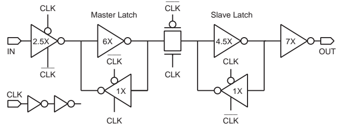
Fig. 3. Schematic diagram of implemented FF.
