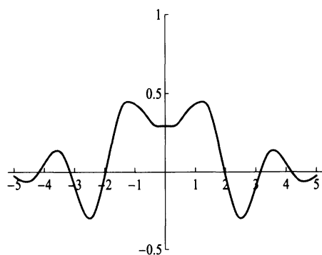
(a) \text{Re } \varphi_2^{ST}
