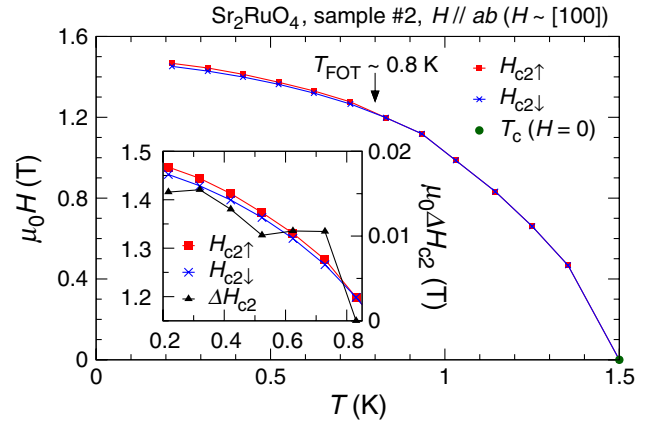
FIG. 4 (color online). Superconducting phase diagram of \text{Sr}_2\text{RuO}_4 for H \parallel ab ( H \sim [100] ) deduced from the MCE for sample 2. The red squares and the blue crosses indicate the onset H_{c2} for the up- and down-sweeps, respectively. The inset presents H_{c2} and \Delta H_{c2} (triangles) in the low-temperature region.
