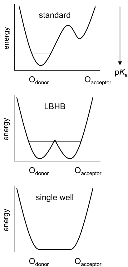
Fig. S1. Overview of typical potential-energy profiles: (Top) standard H-bonds (asymmetric double-well), typically with an O_{\text{donor}}-O_{\text{acceptor}} distance > \sim 2.6 Å; (Middle) low barrier H-bond (LBHB), typically with an O_{\text{donor}}-O_{\text{acceptor}} distance of 2.5–2.6 Å; (Bottom) single-well (ionic) H-bonds, typically with an O_{\text{donor}}-O_{\text{acceptor}} distance of < \sim 2.5 Å (1). The corresponding O–N distances are generally greater than O–O distances.
